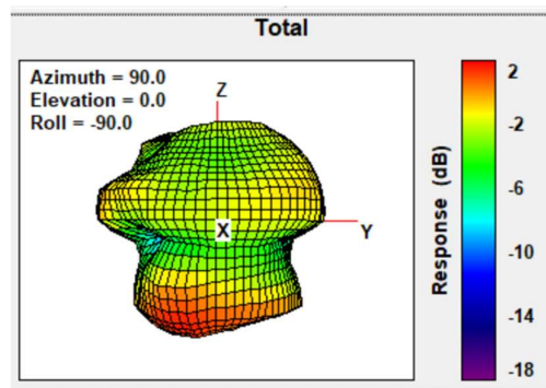
Total Gain Left Side view 2440MHz
