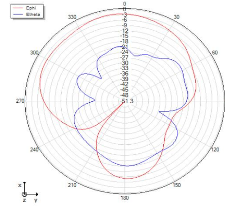
Theta=90 freq=2466MHz
