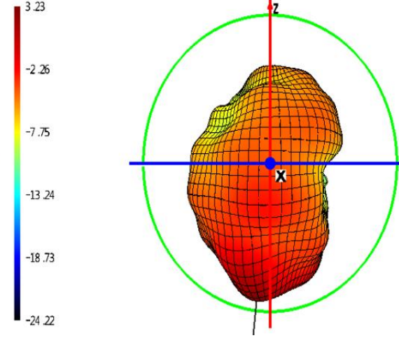
Phi=90 freq=2466MHz
