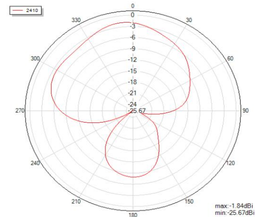
Theta=90 freq=2410MHz
