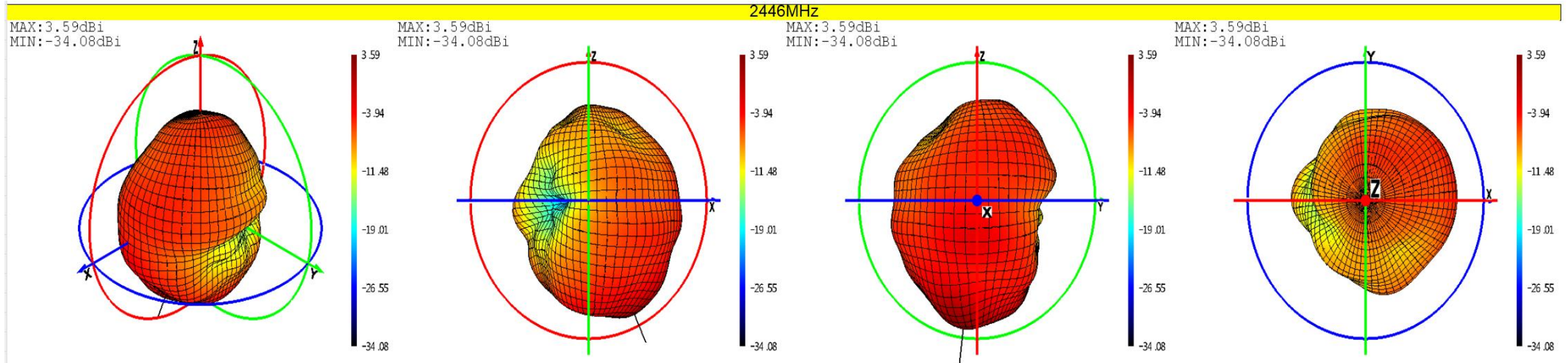
Phi=0 freq=2446MHz
