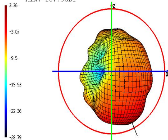
Phi=0 freq=2410MHz
