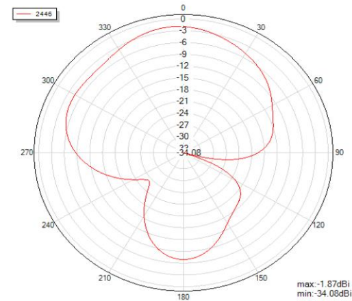
Theta=90 freq=2446MHz
