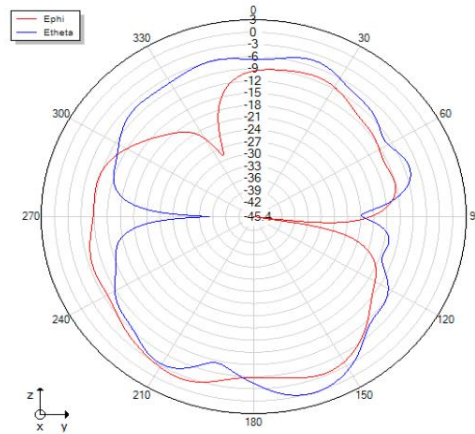
Phi=90 freq=2446MHz
