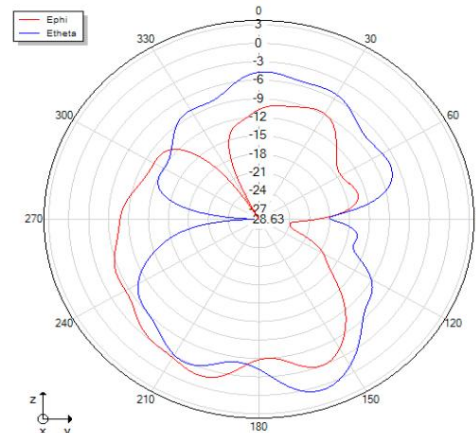
Phi=90 freq=2410MHz
