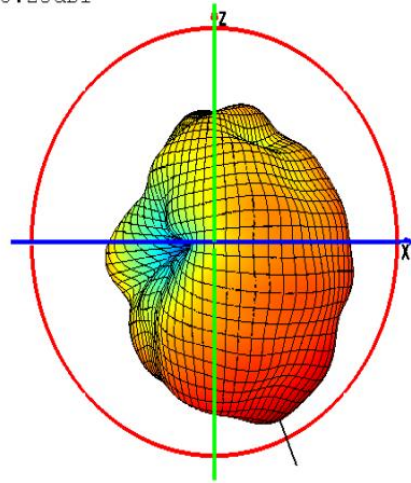
Phi=0 freq=2460MHz
