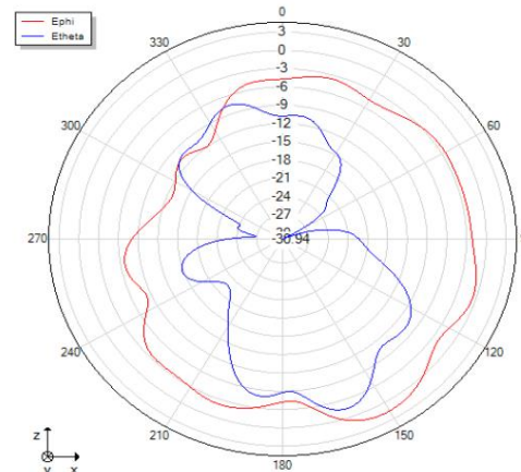
Phi=0 freq=2410MHz
