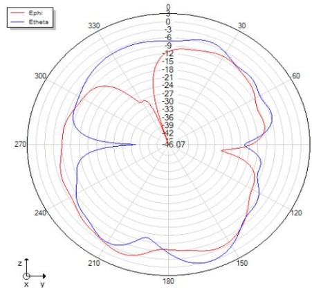
Phi=90 freq=2460MHz
