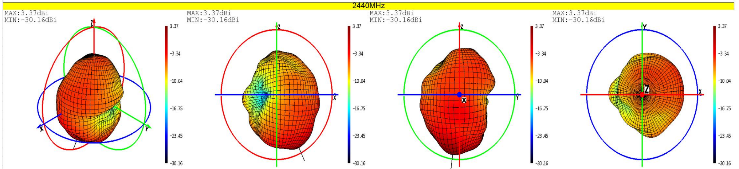
Phi=0 freq=2440MHz
