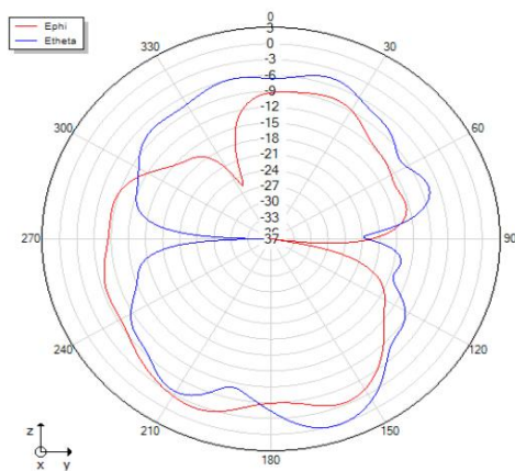
Phi=90 freq=2440MHz
