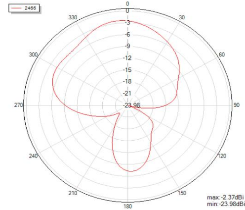
Theta=90 freq=2466MHz
