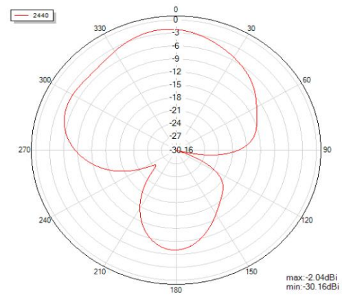
Theta=90 freq=2440MHz
