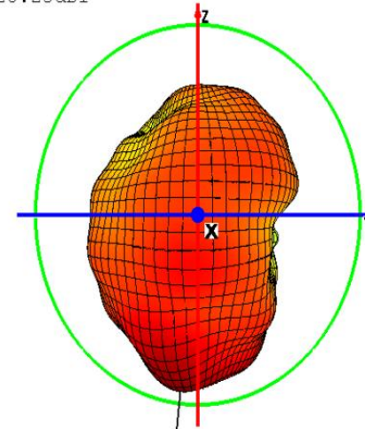
Phi=90 freq=2460MHz
