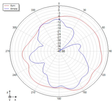
Phi=0 freq=2440MHz
