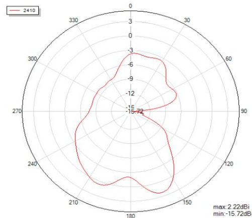
Phi=90 freq=2410MHz
