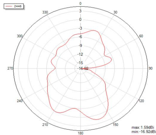
Phi=90 freq=2446MHz
