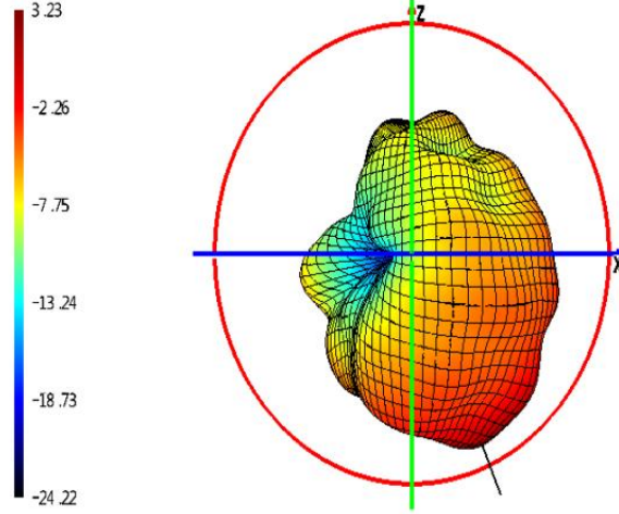
Phi=0 freq=2466MHz
