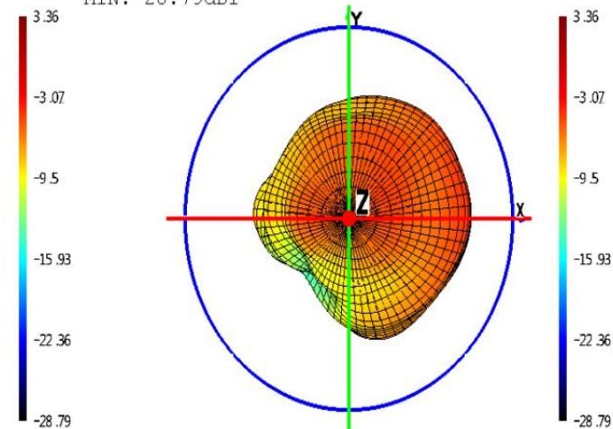
Theta=90 freq=2410MHz
