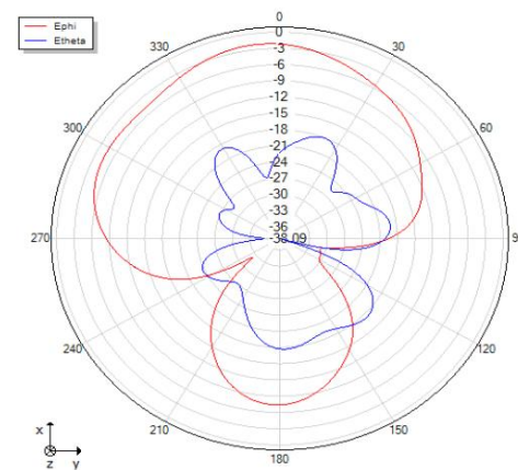
Theta=90 freq=2440MHz
