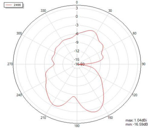
Phi=90 freq=2466MHz
