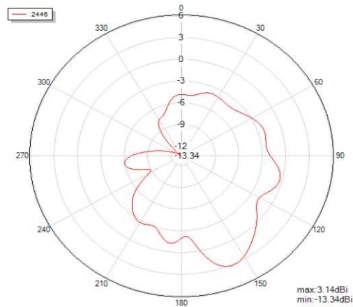
Phi=0 freq=2446MHz
