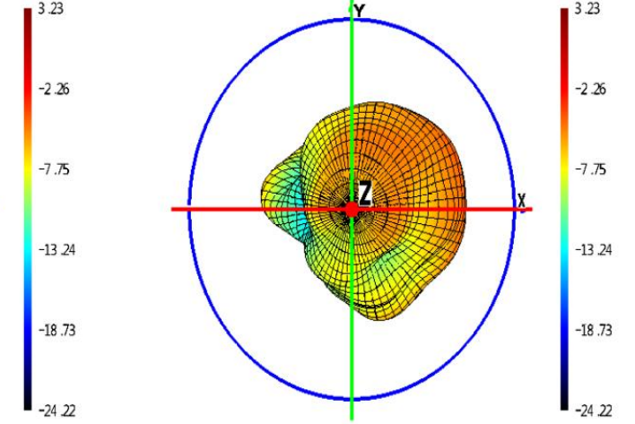
Theta=90 freq=2466MHz
