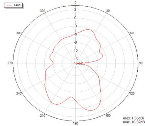
Phi=90 freq=2460MHz
