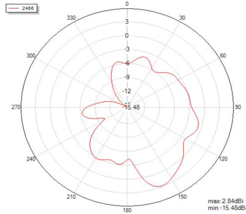
Phi=0 freq=2466MHz
