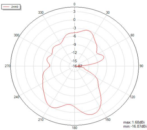
Phi=90 freq=2440MHz
