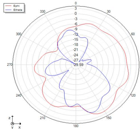
Phi=0 freq=2460MHz
