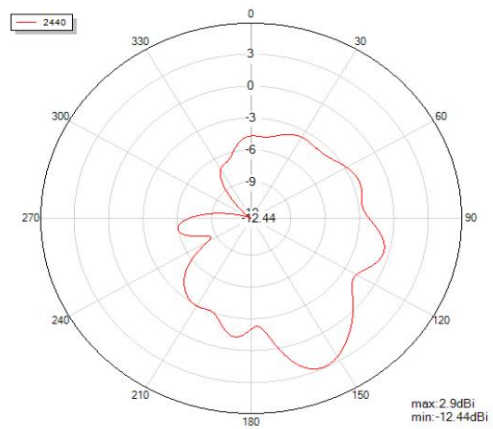
Phi=0 freq=2440MHz
