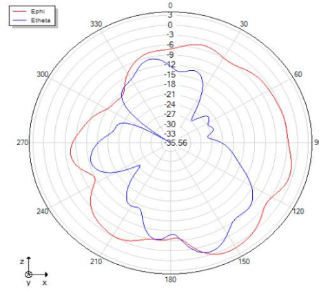
Phi=0 freq=2466MHz
