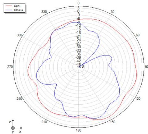
Phi=0 freq=2446MHz
