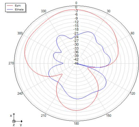
Theta=90 freq=2446MHz
