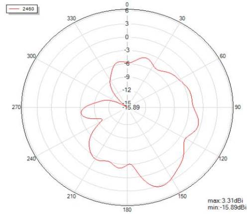
Phi=0 freq=2460MHz
