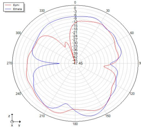
Phi=90 freq=2466MHz
