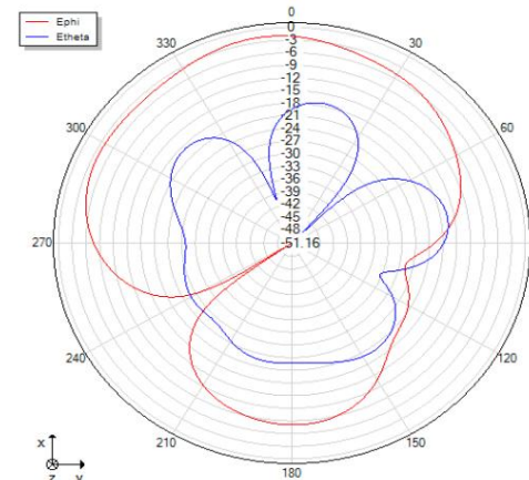
Theta=90 freq=2410MHz
