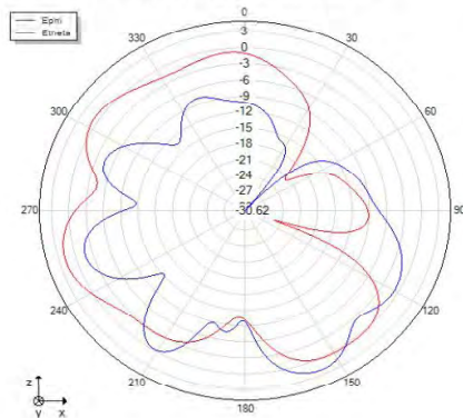
Phi=0 freq=2416MHz
