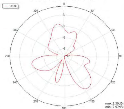
Phi=90 freq=2410MHz
