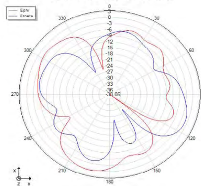
Theta=90 freq=2410MHz
