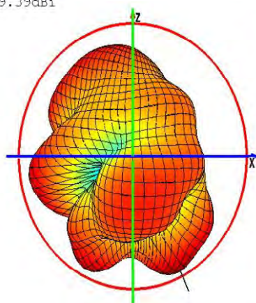
Phi=0 freq=2428MHz
