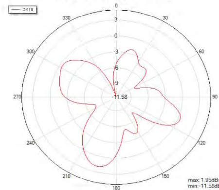
Theta=90 freq=2416MHz
