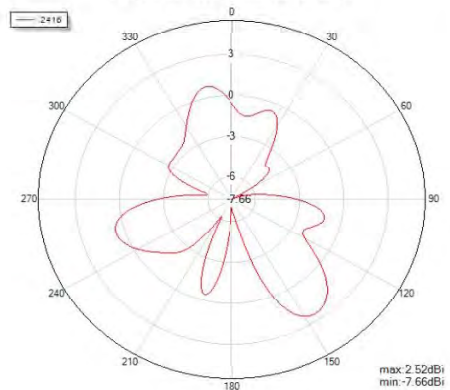
Phi=90 freq=2416MHz
