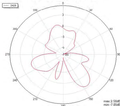
Phi=90 freq=2428MHz
