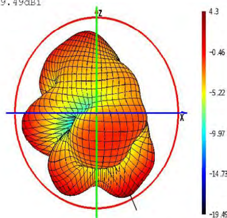
Phi=0 freq=2410MHz
