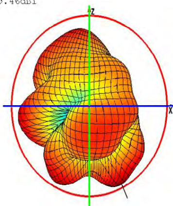
Phi=0 freq=2416MHz
