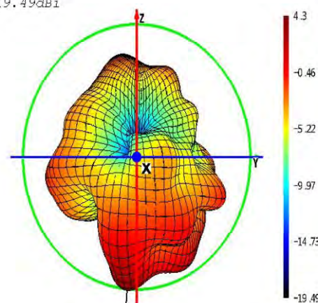
Theta=90 freq=2410MHz
