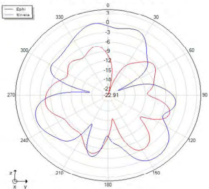
Phi=90 freq=2416MHz
