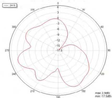
Phi=0 freq=2410MHz
