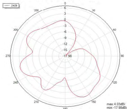
Phi=0 freq=2428MHz
