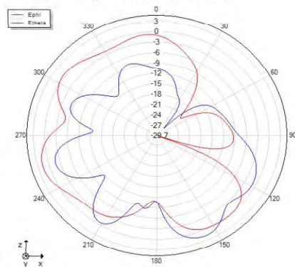
Phi=0 freq=2410MHz
