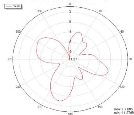
Theta=90 freq=2410MHz
