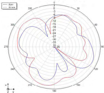
Theta=90 freq=2416MHz
