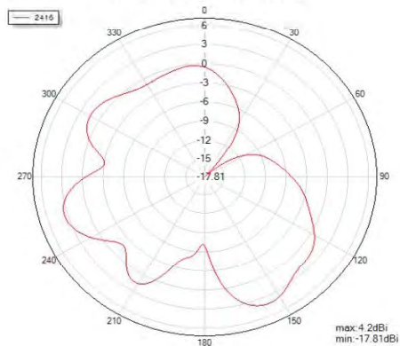
Phi=0 freq=2416MHz
