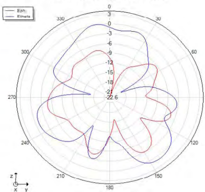
Phi=90 freq=2410MHz
