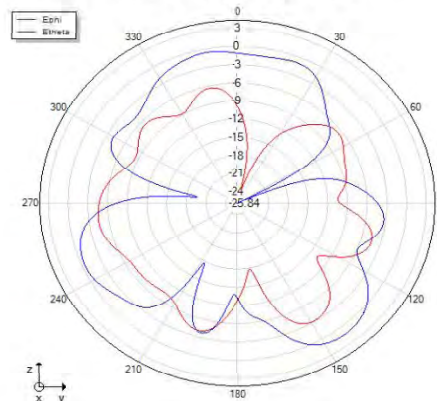
Phi=90 freq=2428MHz
