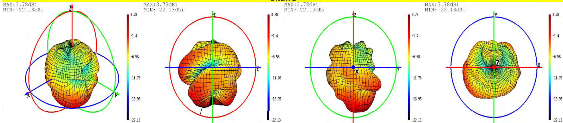
Phi=0 freq=2402MHz
