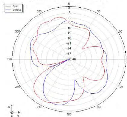
Theta=90 freq=2402MHz
