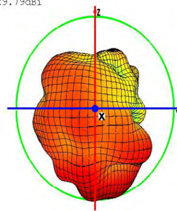
Theta=90 freq=2480MHz
