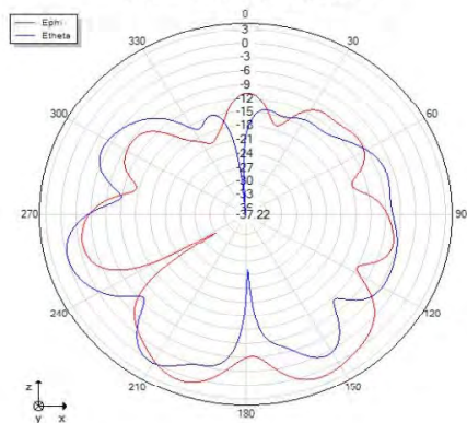
Phi=0 freq=2402MHz
