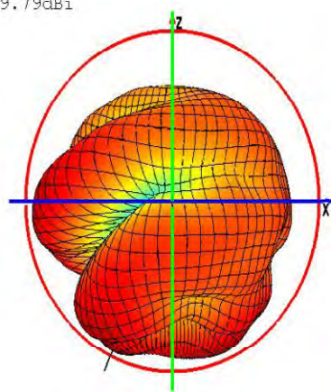
Phi=0 freq=2480MHz
