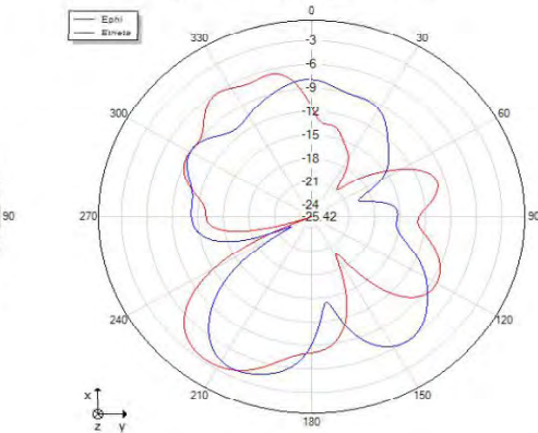
Theta=90 freq=2480MHz
