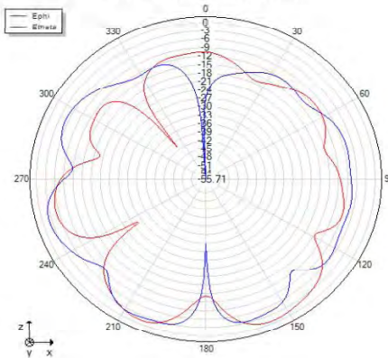
Phi=0 freq=2480MHz
