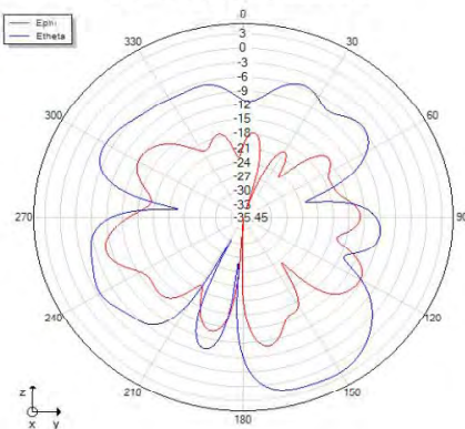
Phi=90 freq=2402MHz
