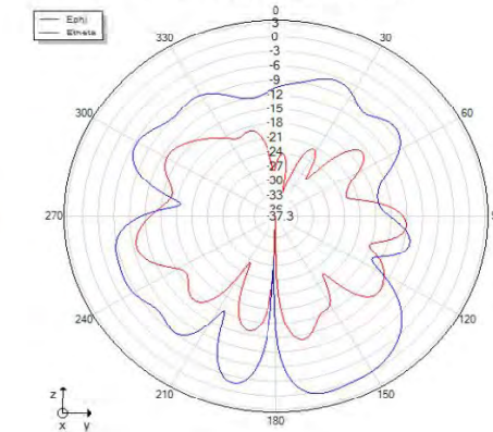
Phi=90 freq=2480MHz
