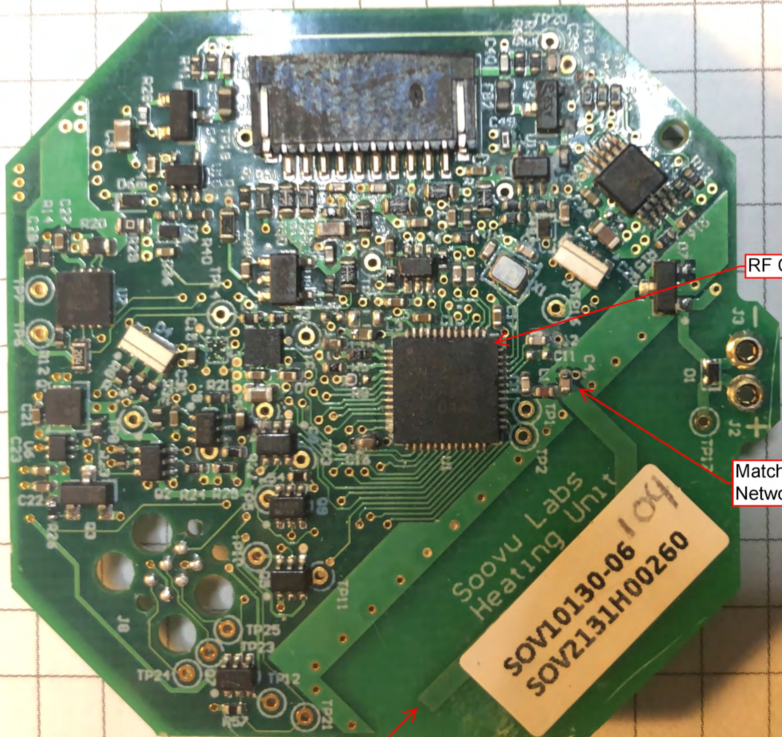
RF Antenna
