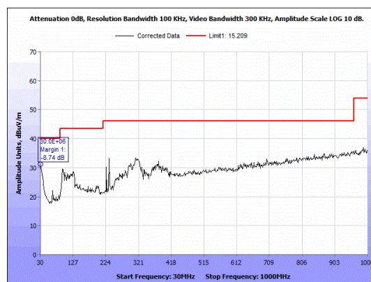
Figure 24: Radiated Spurious Emissions, 2440 MHz - 30-1000 MHz - Horizontal.
