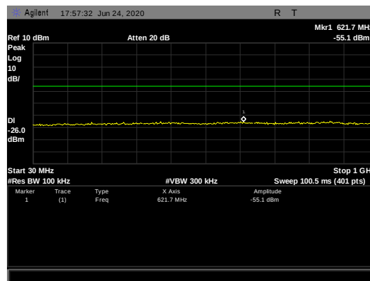
Figure 45: Conducted Spurious Emissions, 2440 MHz - 30-1000 MHz
