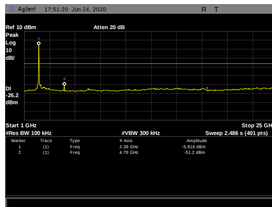
Figure 44: Conducted Spurious Emissions, 2402 MHz - 1-25 GHz
