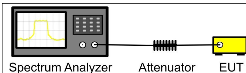
Figure 14. Power Output Test Setup
