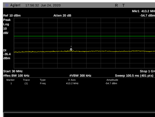
Figure 47: Conducted Spurious Emissions, 2480 MHz - 30-1000 MHz
