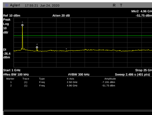
Figure 48: Conducted Spurious Emissions, 2480 MHz - 1-25 GHz
