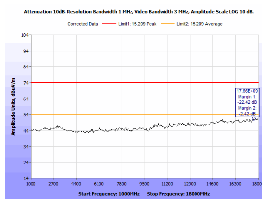
Figure 23: Radiated Spurious Emissions, 2440 MHz - 1-18 GHz - Peak - Horizontal.
