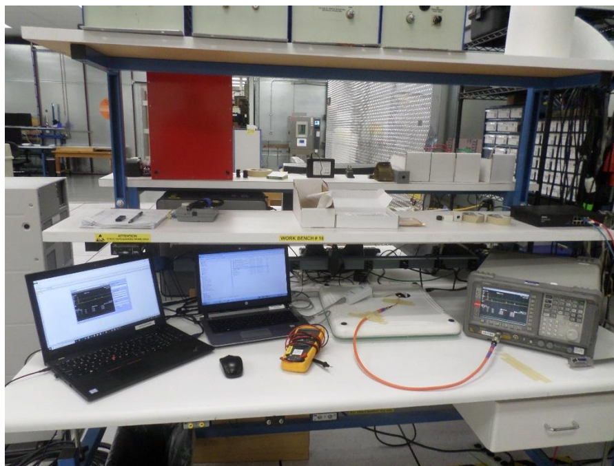
Figure 49: Conducted Spurious Emissions, Setup Photo
