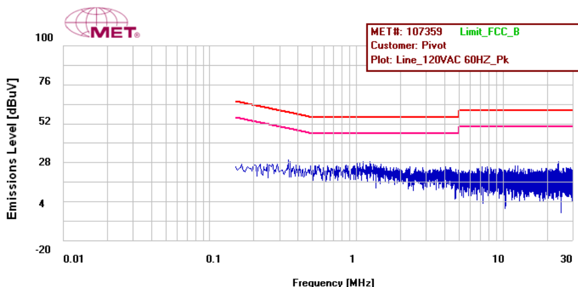
Figure 2: Conducted Emissions, 15.207(a), Phase Line
