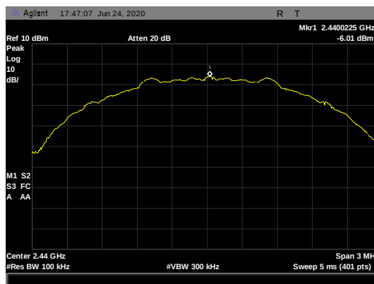
Figure 51: Peak Power Spectral Density, 2440 MHz - (-6.01 dBm)
