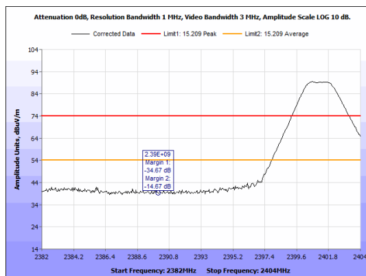
Figure 32: Radiated Band Edge, 2402 MHz - Peak - Vertical.
