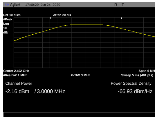
Figure 15: Peak Output Power, 2402 MHz - (-2.16 dBm)
