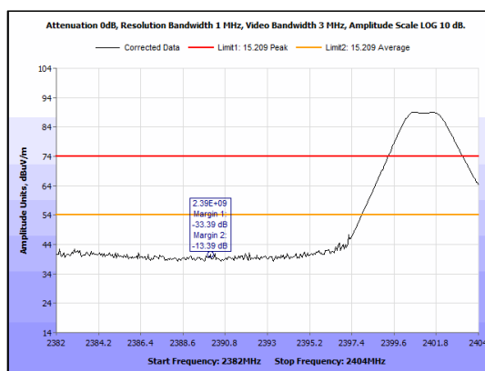
Figure 31: Radiated Band Edge, 2402 MHz - Peak - Horizontal.
