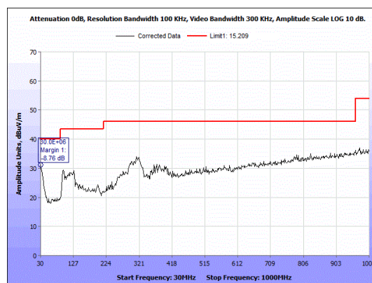
Figure 27: Radiated Spurious Emissions, 2480 MHz - 30-1000 MHz - Horizontal.
