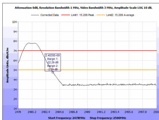
Figure 33: Radiated Band Edge, 2480 MHz - Peak - Horizontal.
