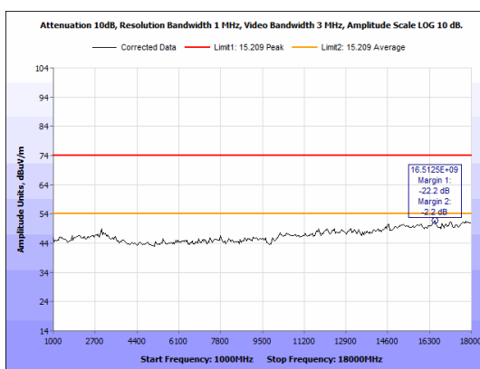
Figure 21: Radiated Spurious Emissions, 2402 MHz - 1-18 GHz - Peak - Horizontal.
