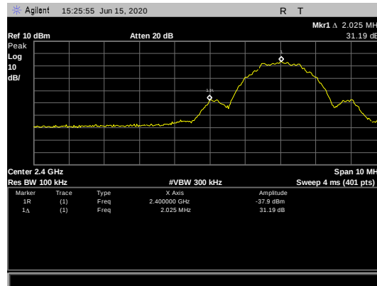
Figure 41: Conducted Band Edge, 2402 MHz
