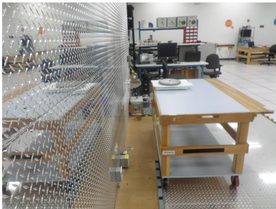
Figure 6. Conducted Emissions, 15.207(a), Test Setup, Rear View
