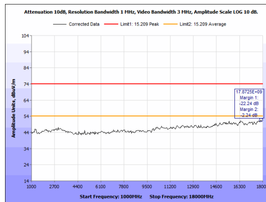
Figure 26: Radiated Spurious Emissions, 2440 MHz - 1-18 GHz - Peak - Vertical.
