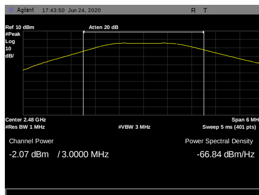
Figure 17: Peak Output Power, 2480 MHz - (-2.07 dBm)
