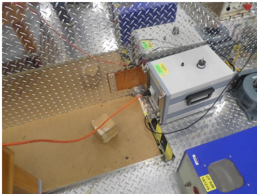
Figure 5. Conducted Emissions, 15.207(a), Test Setup, LISN View
