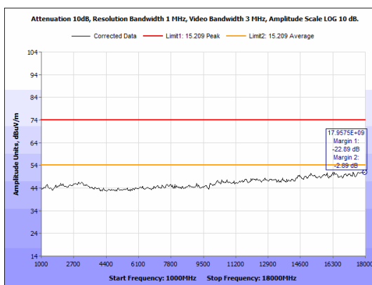
Figure 30: Radiated Spurious Emissions, 2480 MHz - 1-18 GHz - Peak - Vertical.
