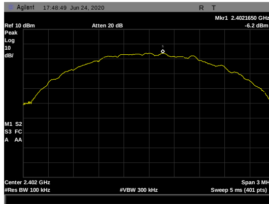
Figure 50: Peak Power Spectral Density, 2402 MHz - (-6.2 dBm)
