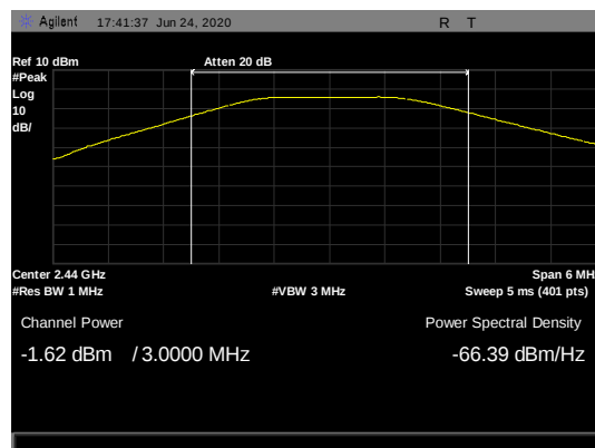
Figure 16: Peak Output Power, 2440 MHz - (-1.62 dBm)
