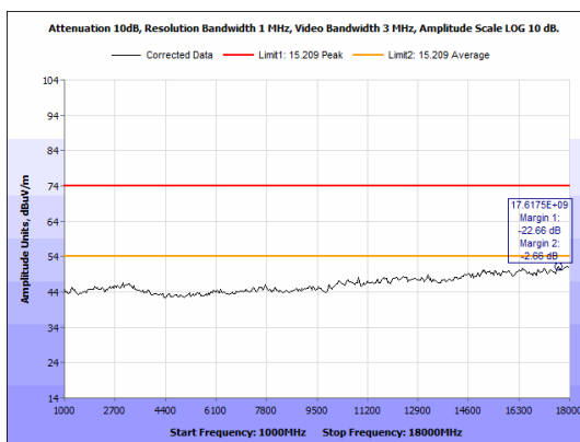
Figure 29: Radiated Spurious Emissions, 2480 MHz - 1-18 GHz - Peak - Horizontal.
