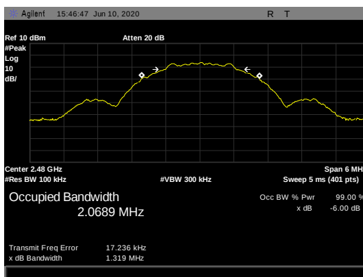
Figure 10: 6 dB Occupied Bandwidth, 2480 MHz - 1.319 MHz
