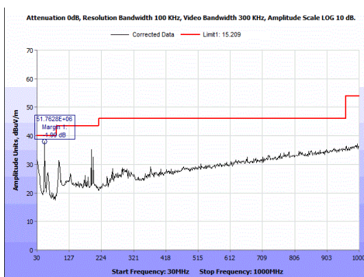
Figure 20: Radiated Spurious Emissions, 2402 MHz - 30-1000 MHz - Vertical.
