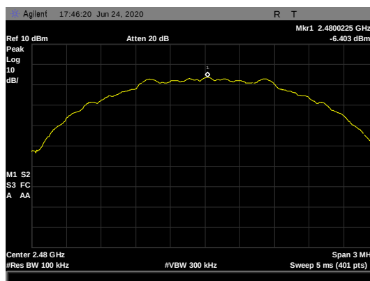
Figure 52: Peak Power Spectral Density, 2480 MHz - (-6.403 dBm)
