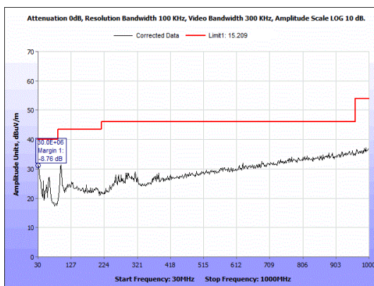
Figure 28: Radiated Spurious Emissions, 2480 MHz - 30-1000 MHz - Vertical.
