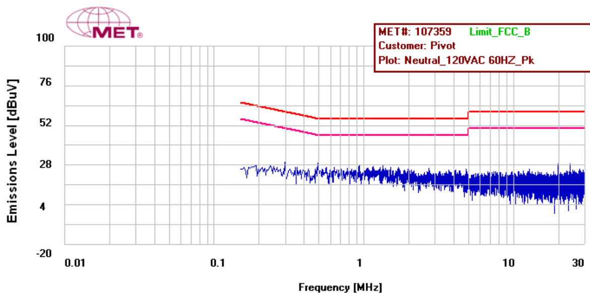
Figure 3: Conducted Emissions, 15.207(a), Neutral Line
