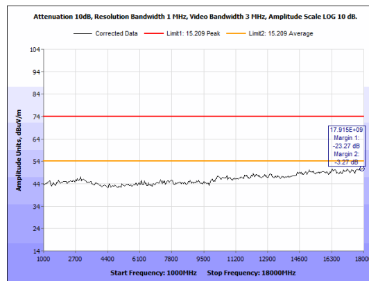
Figure 22: Radiated Spurious Emissions, 2402 MHz - 1-18 GHz - Peak - Vertical.
