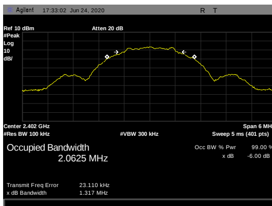
Figure 8: 6 dB Occupied Bandwidth, 2402 MHz - 1.317 MHz
