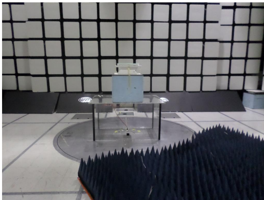
Figure 39: Radiated Emissions - 1-18 GHz- Setup Front View
