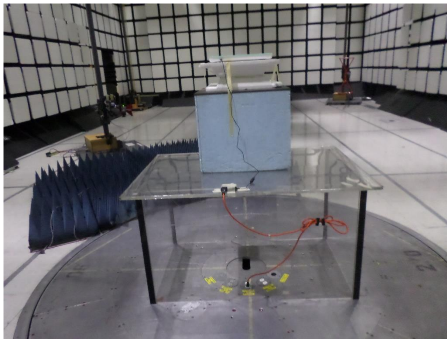
Figure 40: Radiated Emissions - 1-18 GHz- Setup Rear View
