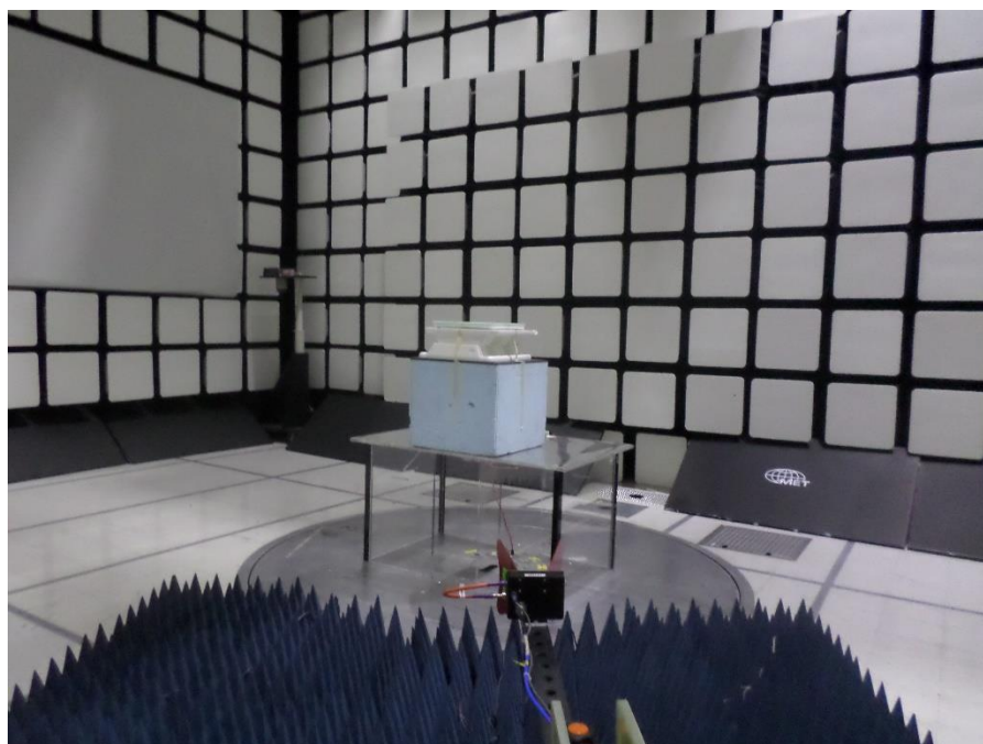
Figure 38: Radiated Emissions - 1-18 GHz- Setup Antenna View
