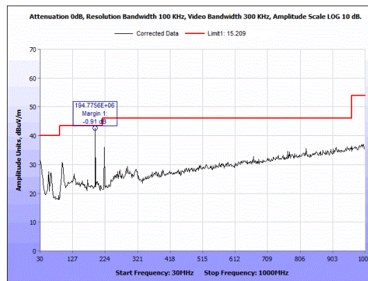
Figure 25: Radiated Spurious Emissions, 2440 MHz - 30-1000 MHz - Vertical.
