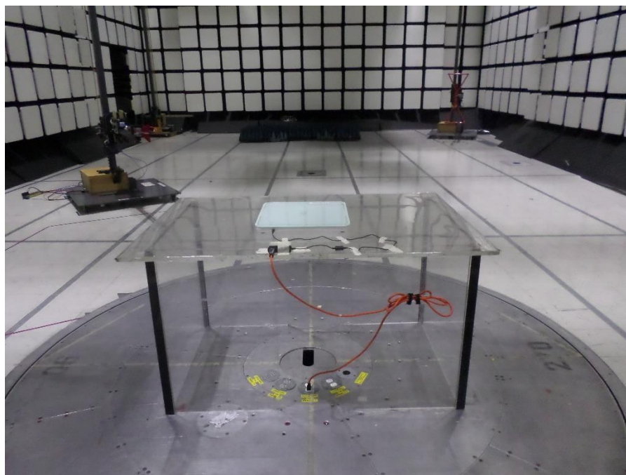
Figure 37: Radiated Emissions - 30-1000 MHz- Setup Rear View
