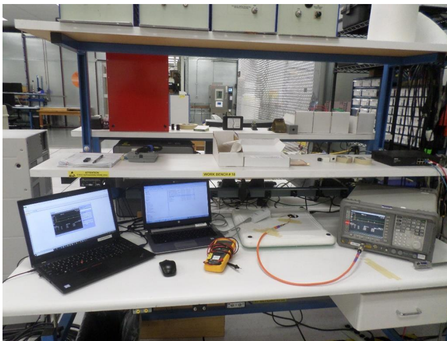
Figure 13: Duty Cycle, Setup Photo
