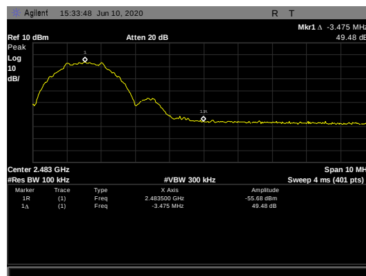
Figure 42: Conducted Band Edge, 2480 MHz
