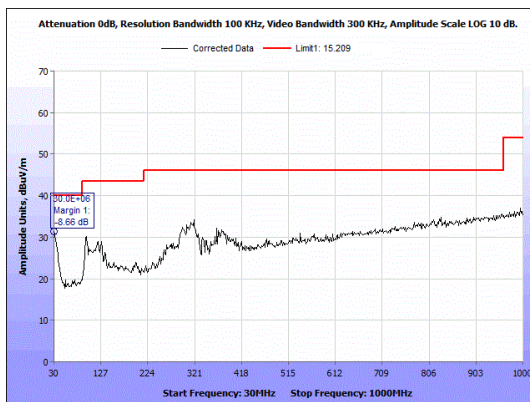
Figure 19: Radiated Spurious Emissions, 2402 MHz - 30-1000 MHz - Horizontal.
