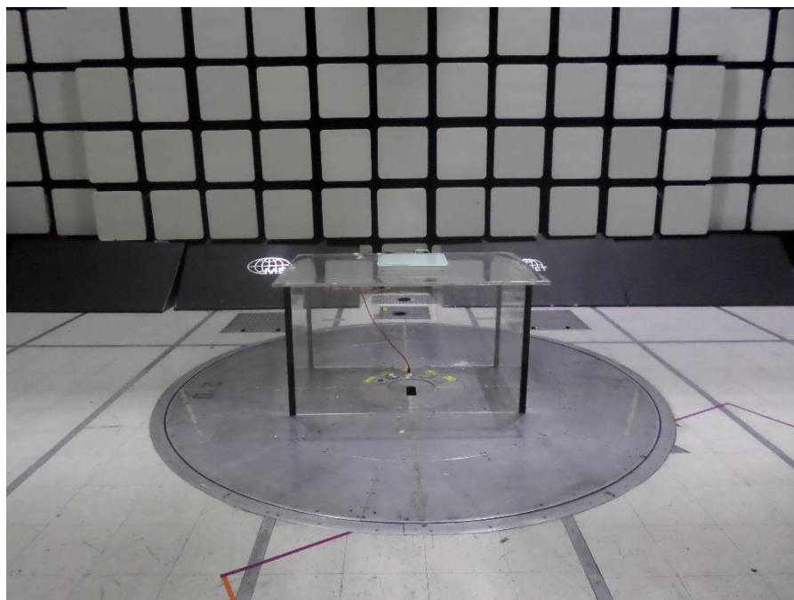
Figure 36: Radiated Emissions - 30-1000 MHz- Setup Front View
