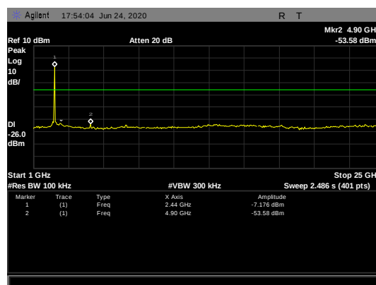
Figure 46: Conducted Spurious Emissions, 2440 MHz - 1-25 GHz
