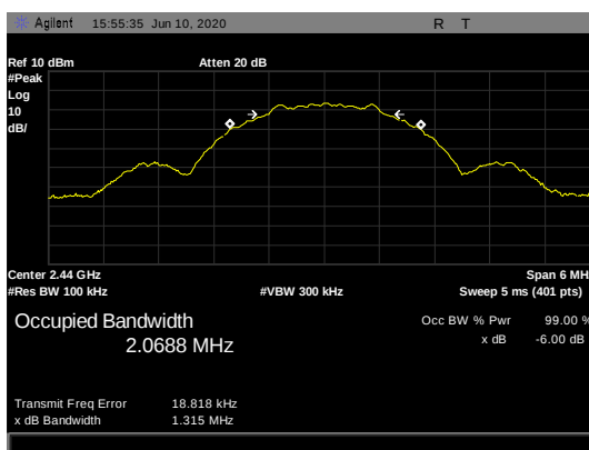
Figure 9: 6 dB Occupied Bandwidth, 2440 MHz - 1.315 MHz
