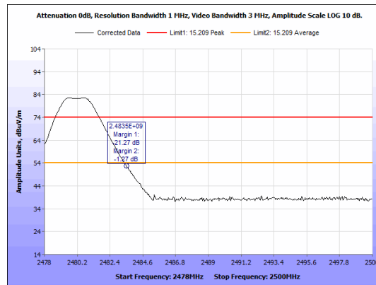
Figure 34: Radiated Band Edge, 2480 MHz - Peak - Vertical.
