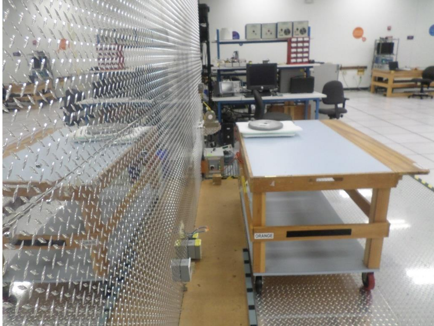
Figure 3. Conducted Emissions, 15.207(a), Test Setup, Rear View
