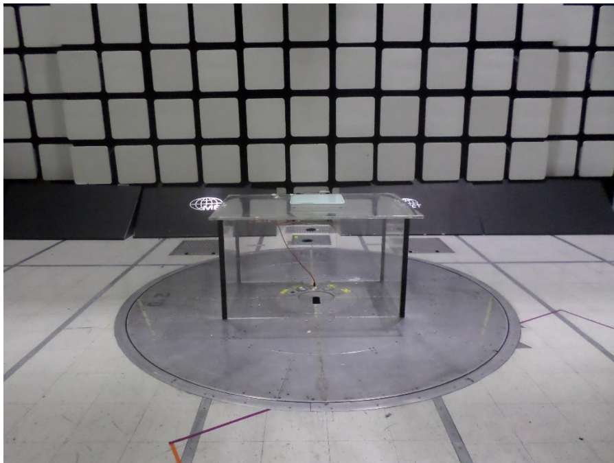
Figure 5: Radiated Emissions - 30-1000 MHz- Setup Front View
