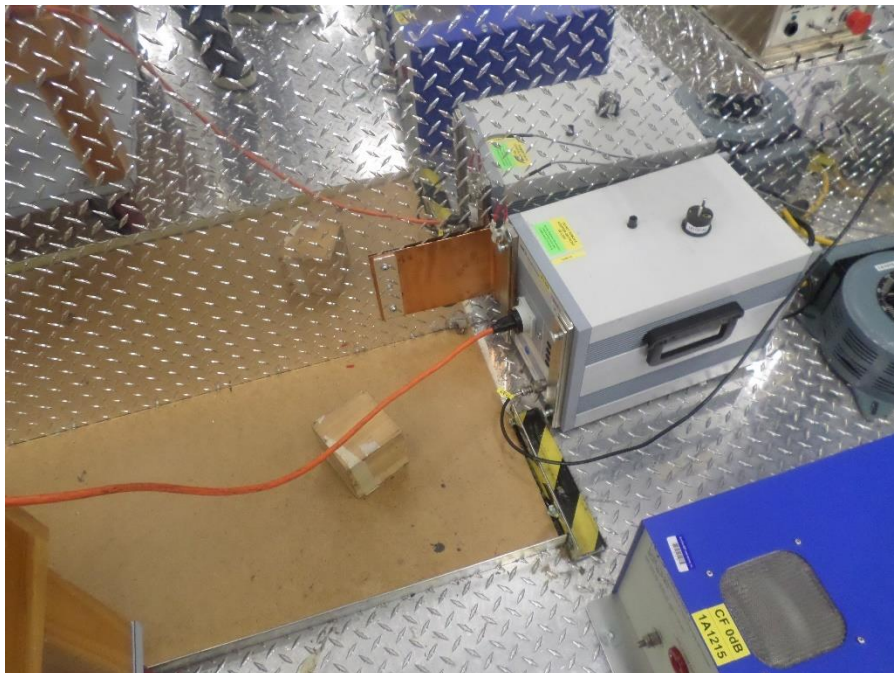
Figure 2. Conducted Emissions, 15.207(a), Test Setup, LISN View
