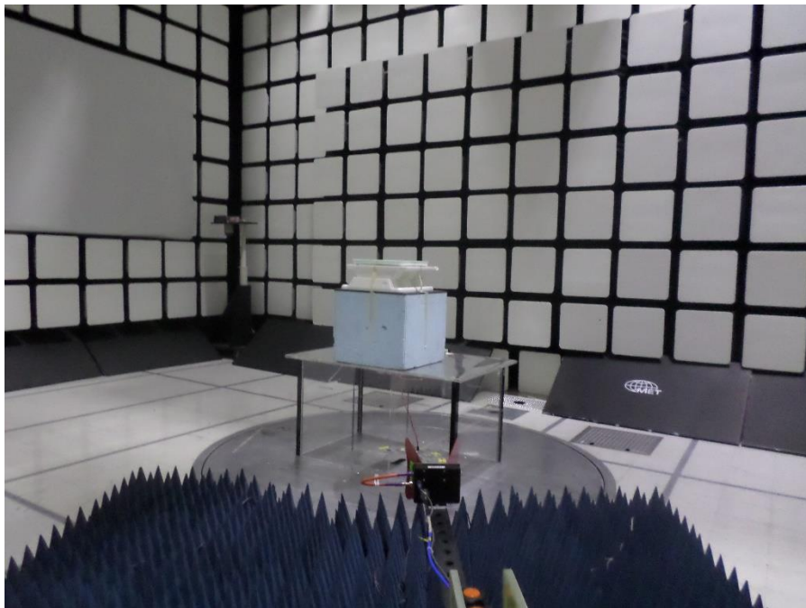
Figure 7: Radiated Emissions - 1-18 GHz- Setup Antenna View
