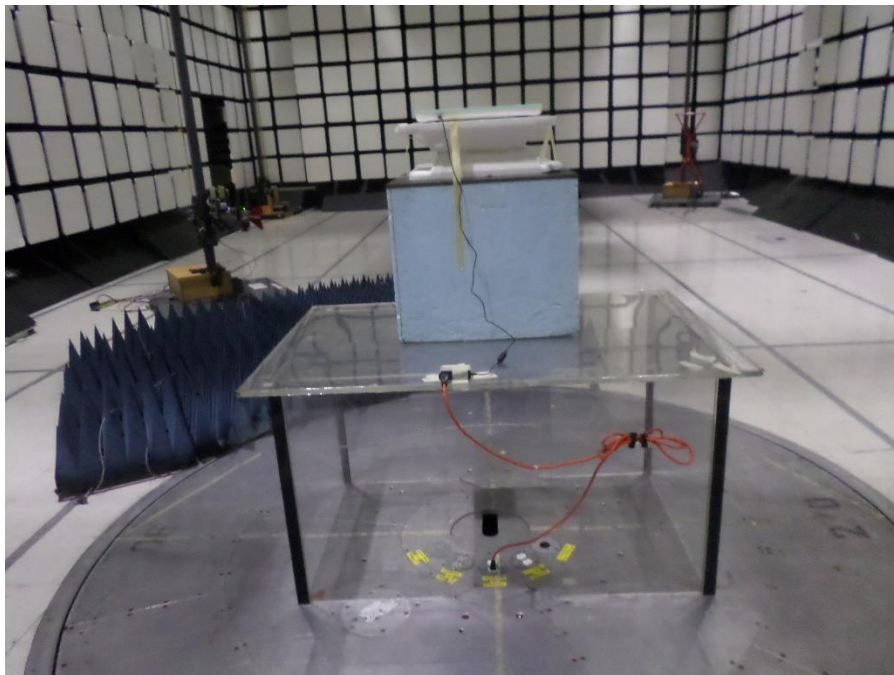
Figure 9: Radiated Emissions - 1-18 GHz- Setup Rear View
