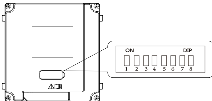
Figure 3-1 DIP Switch
