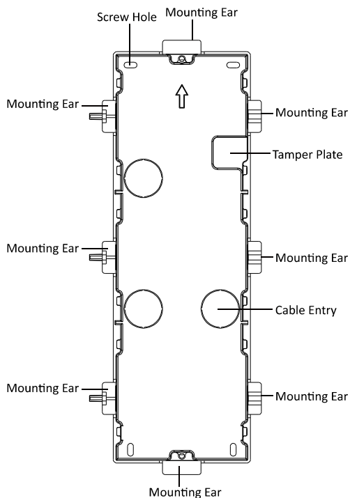
Figure 3-38 Appearance Description
