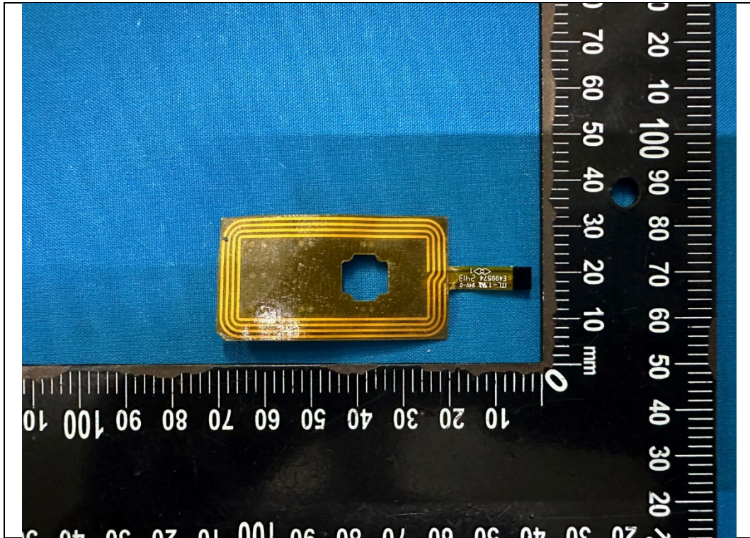
13.56MHz antenna
