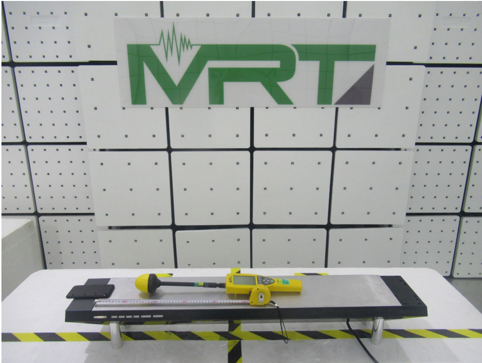
Description: MPE Test Setup
