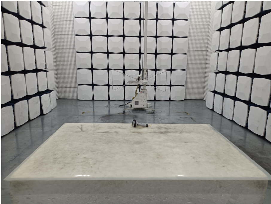
Radiated spurious
