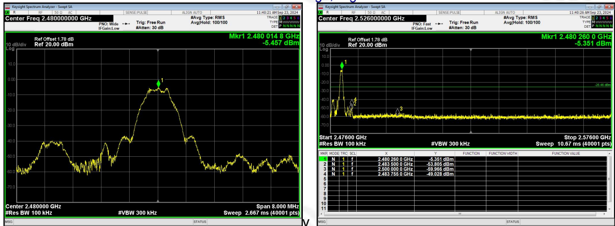
GFSK: Band Edge, Right Side
