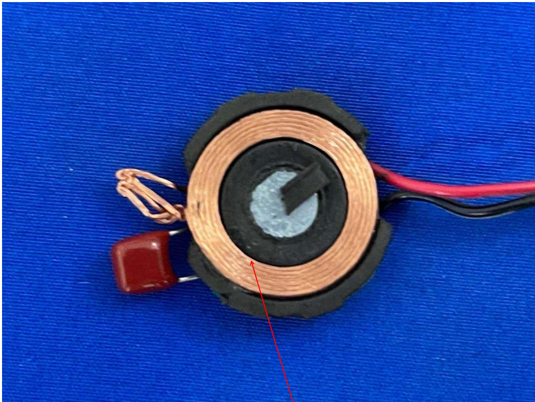
Watch Antenna 2
