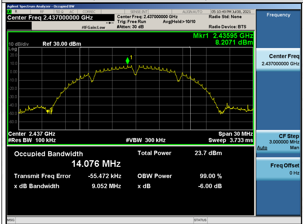
Test_Graph_802.11b_ANT1_2437_1Mbps_DTBSW
