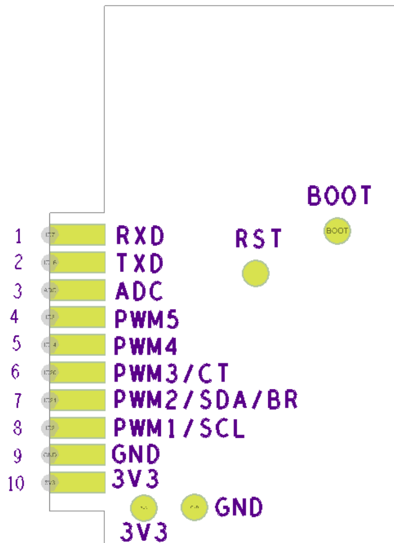
Bottom view
