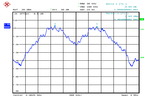
GFSK_Low 1.001MHz
