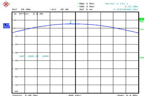
\pi/4 -DQPSK_High 5.22dBm
