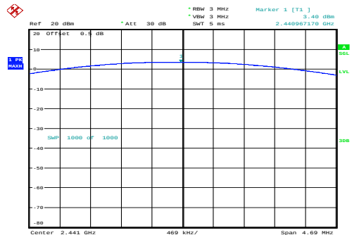
GFSK_Middle 3.40dBm
