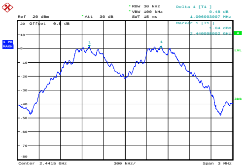
GFSK_Middle 1.007MHz
