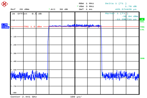
\pi/4 -DQPSK_Hopping_2DH1 0.426ms
