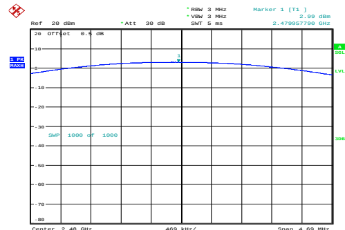
GFSK_High 2.99dBm
