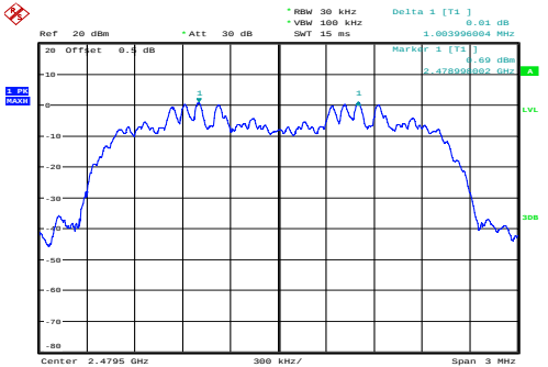
\pi/4 -DQPSK_High 1.004MHz
