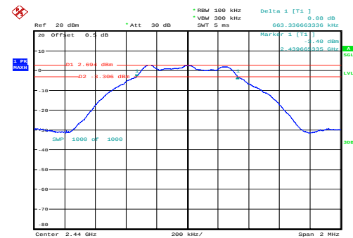
Middle 0.663MHz
