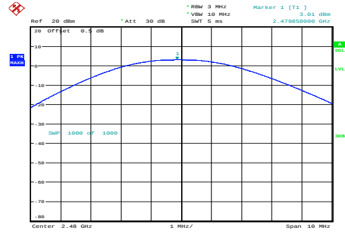
High 3.01dBm
