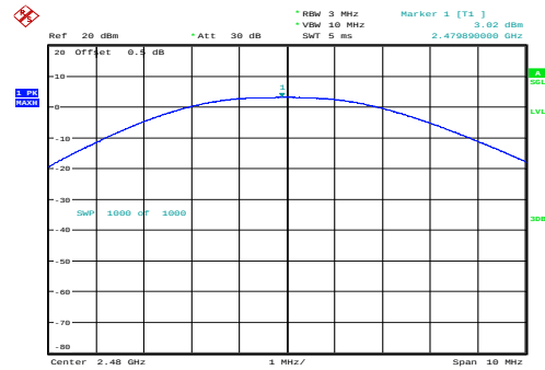
High 3.02dBm
