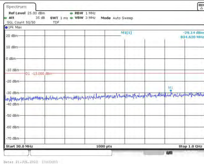
Band66-1.4MHz-QPSK-131979-6RB#0-Range1:30~1000MHz
