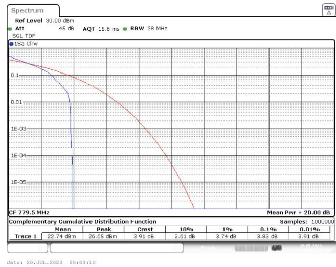
Band13-5MHz-QPSK-23205-25RB#0
