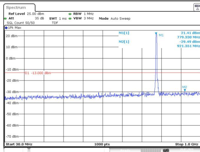
Band13-5MHz-QPSK-23205-25RB#0-Range1:30~1000MHz
