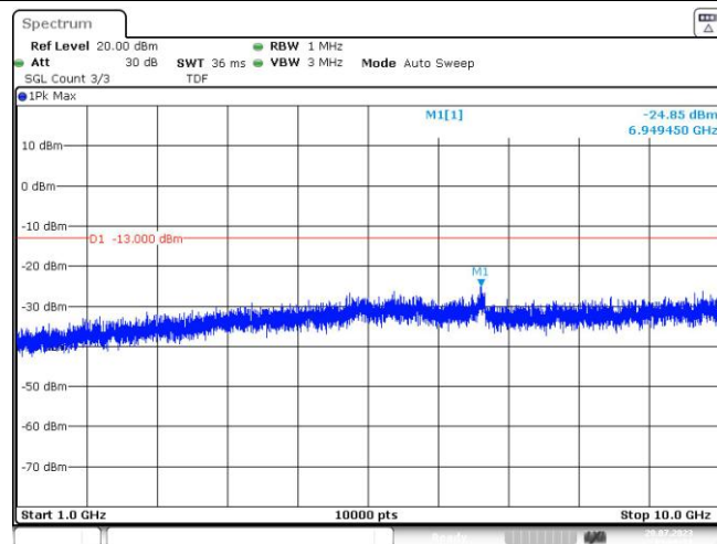
Band13-5MHz-QPSK-23205-1RB#0-Range2:1000~10000MHz
