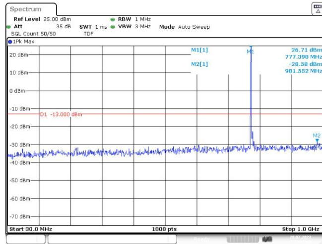
Band13-5MHz-QPSK-23205-1RB#0-Range1:30~1000MHz
