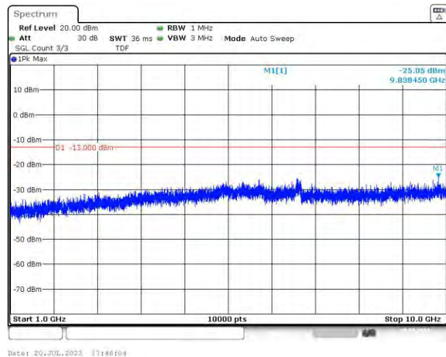
Band5-3MHz-16QAM-20525-15RB#0-Range1:30~1000MHz
