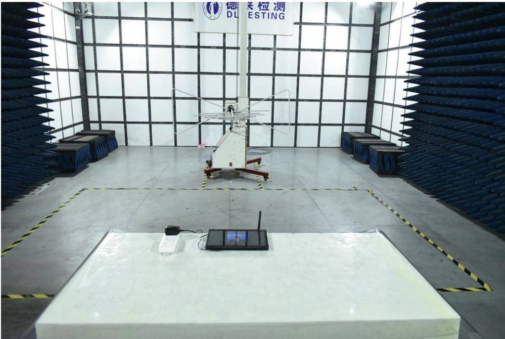
Radiated Emission
