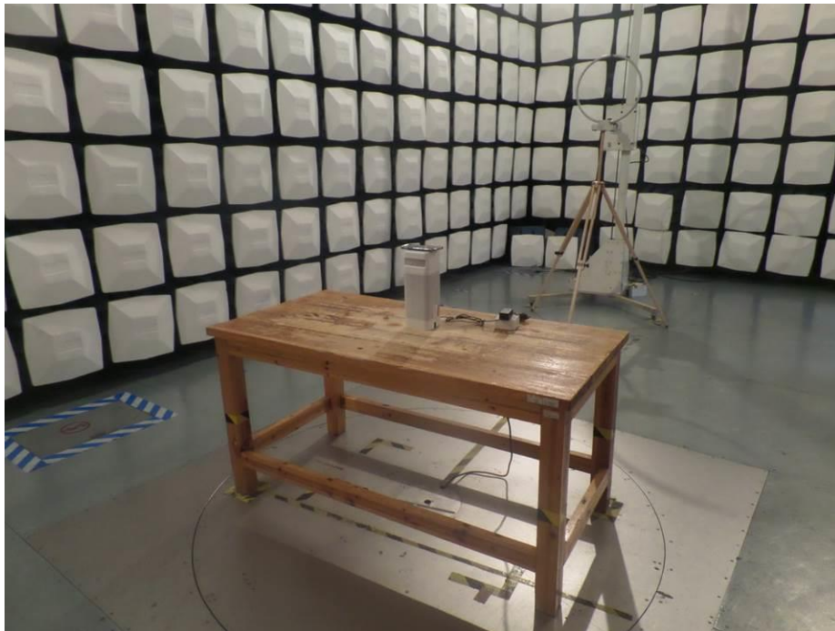
Test Setup For Magnetic Field Disturbance
