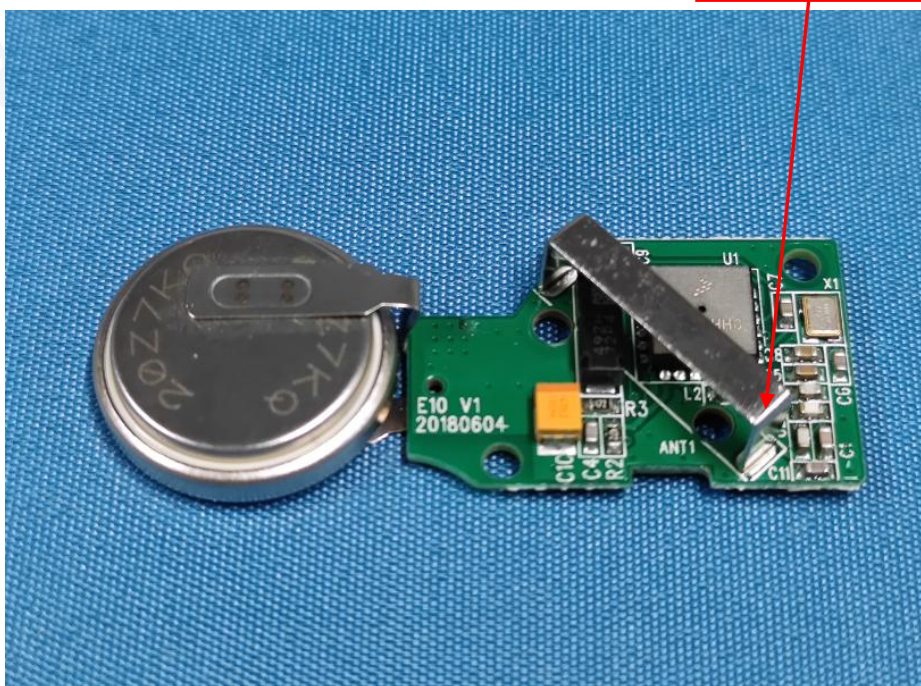
Metal Antenna
