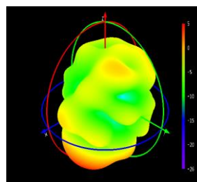
Theta=90 freq=2440MHz
