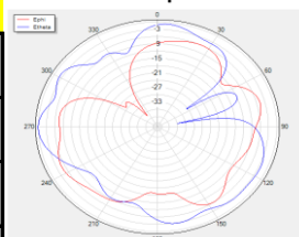
Phi=90 freq=2440MHz
