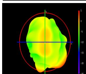
Phi=90 freq=2440MHz
