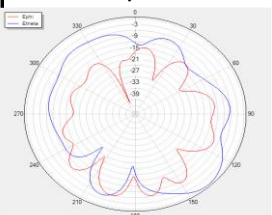
Phi=0 freq=2440MHz
