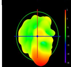
Phi=0 freq=2440MHz
