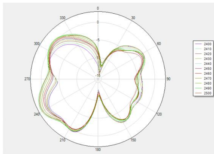
Theta 90 2D
