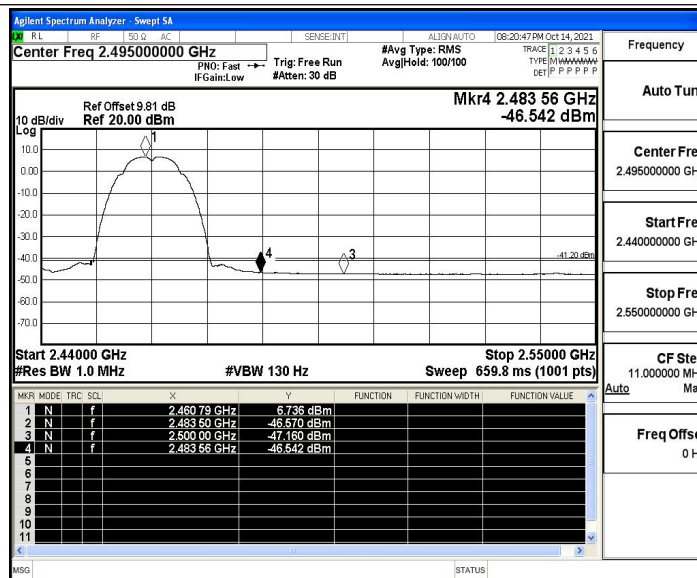
11B_Ant4_High_2462_Peak
