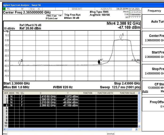
11G_Ant4_Low_2412_AV
