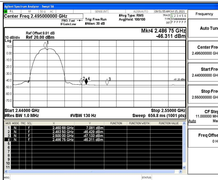
11B_Ant3_High_2462_Peak
