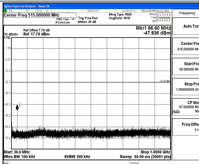
11N20SISO_Ant4_2412_30~1000
