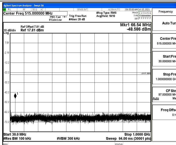
11N40SISO_Ant4_2452_30~1000
