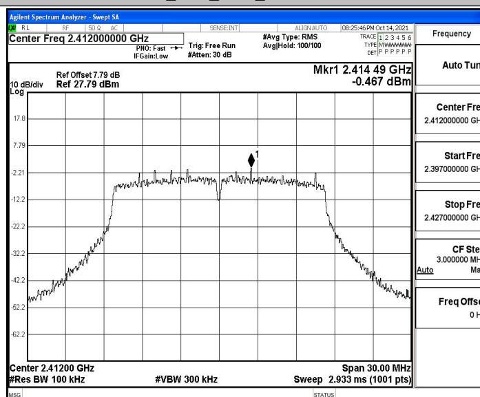
11G_Ant4_2412_0~Reference
