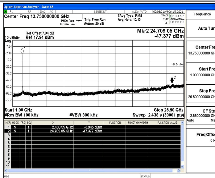
11G_Ant4_2437_1000~26500
