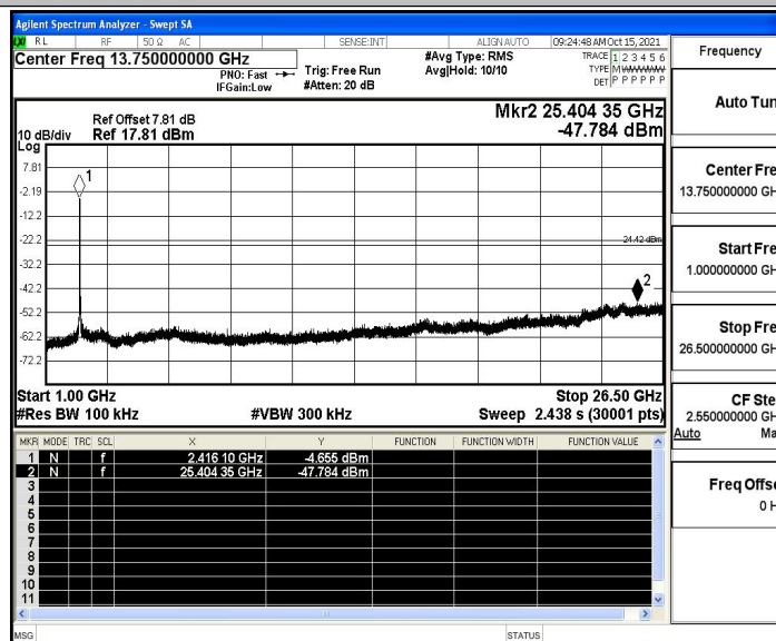
11N40SISO_Ant4_2422_1000~26500
