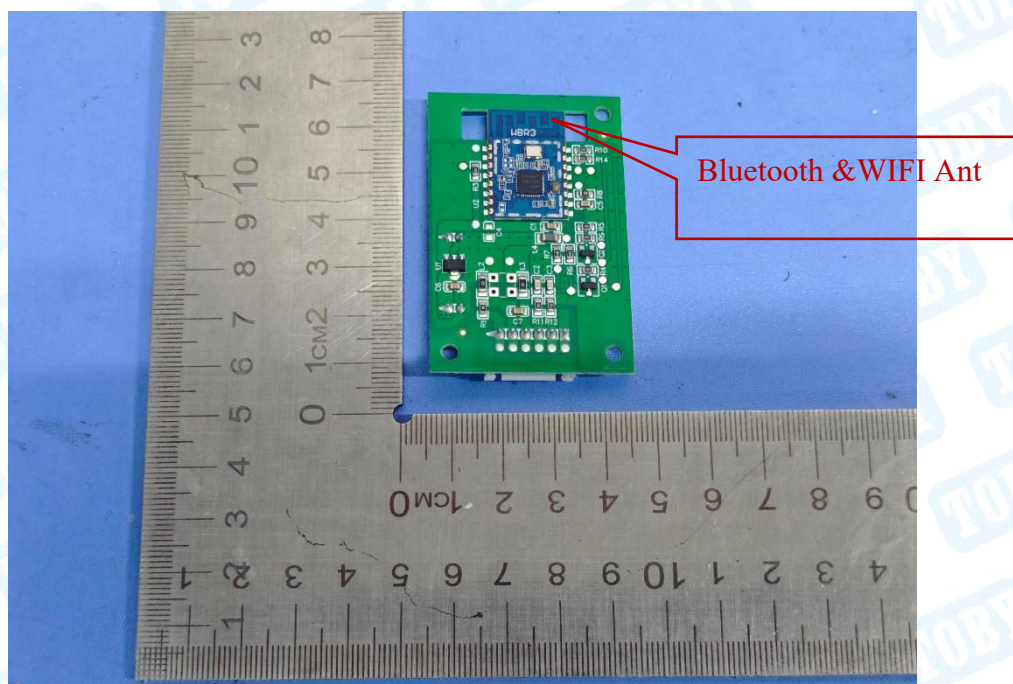
Photo 20 Internal of EUT
