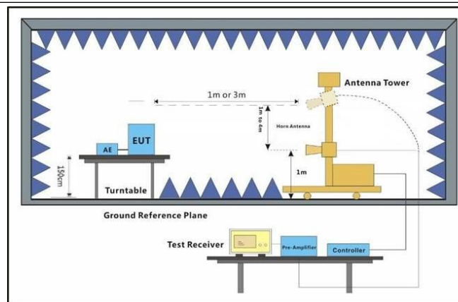
Figure 3. Above 1 GHz
