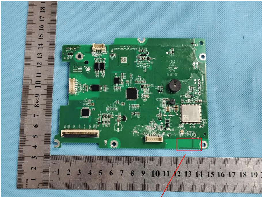
Onboard PCB antenna
