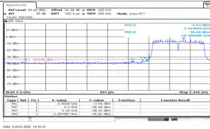
11N40SISO_Ant1_Low_2422
