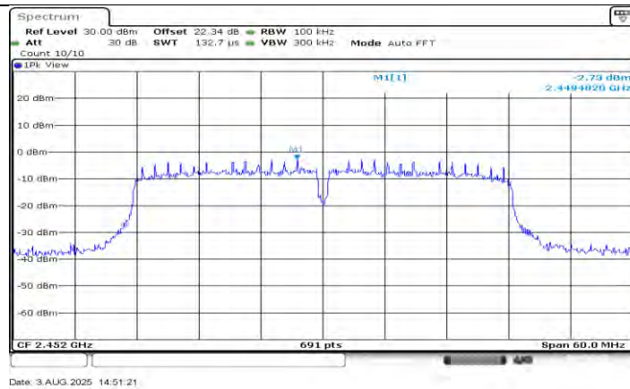
11N40SISO_Ant1_2452_0-Reference
