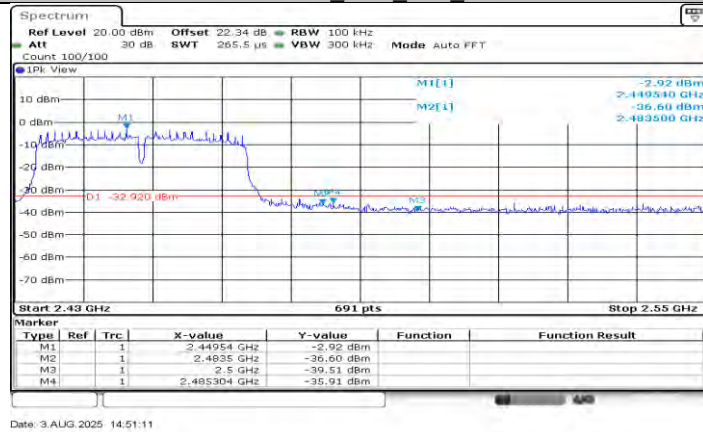
11N40SISO_Ant1_High_2452
