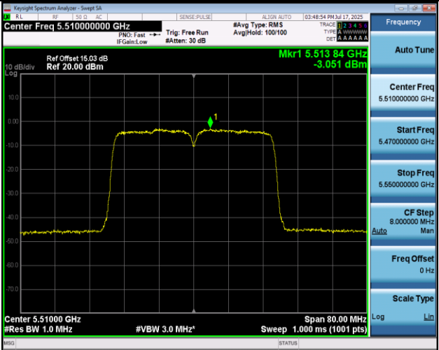
11AC40MIMO-Ant1-5510-PASS
