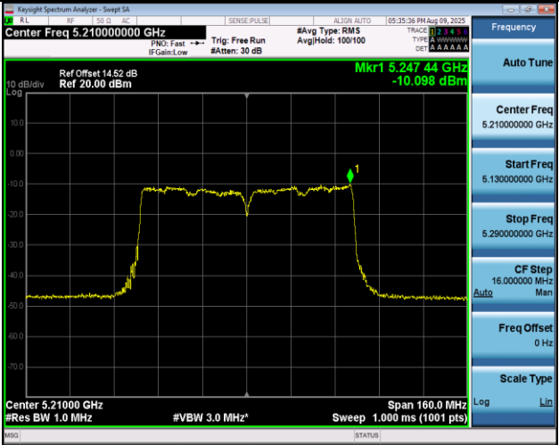
11AC80MIMO-Ant2-5210-PASS
