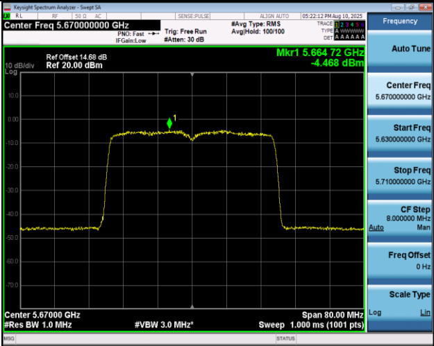
11AX40MIMO-Ant1-5670-PASS
