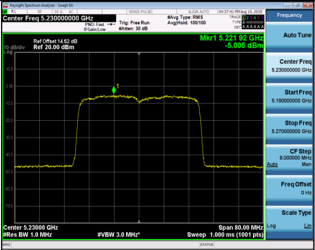
11AX40MIMO-Ant2-5230-PASS
