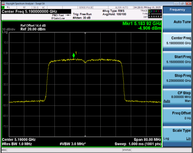
11AX40MIMO-Ant2-5190-PASS
