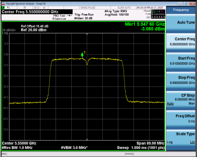
11AC40MIMO-Ant2-5550-PASS
