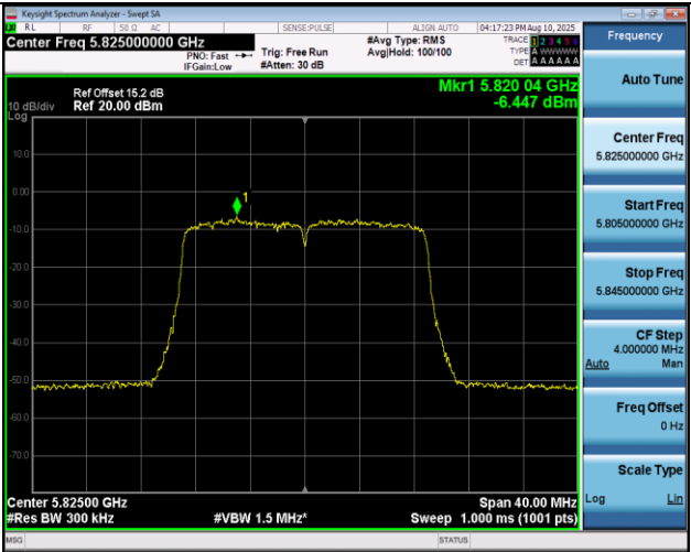
11AX20MIMO-Ant2-5825-PASS
