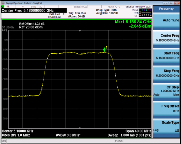
11AX20MIMO-Ant1-5180-PASS
