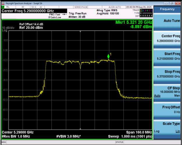
11AC80MIMO-Ant1-5290-PASS
