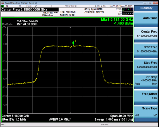
11AX20MIMO-Ant2-5180-PASS
