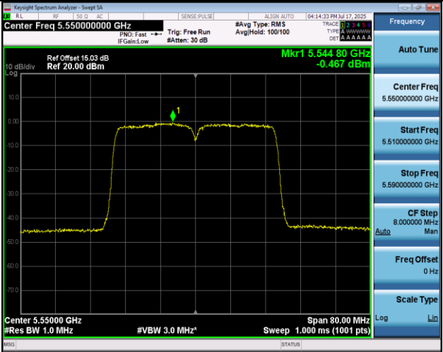
11AC40MIMO-Ant1-5550-PASS
