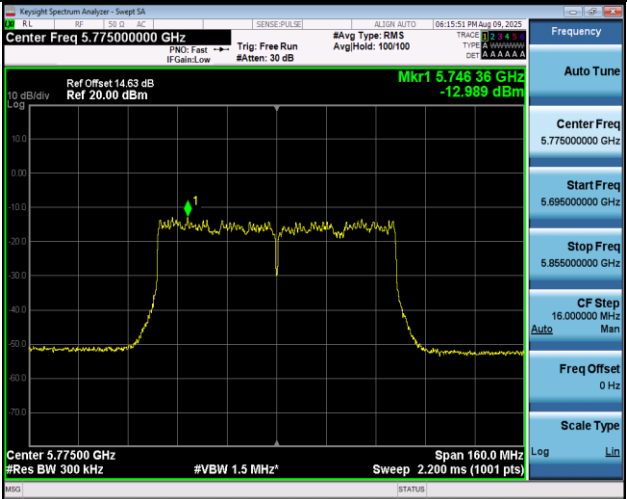
11AC80MIMO-Ant1-5775-PASS
