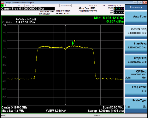
11AX40MIMO-Ant1-5190-PASS
