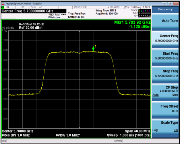
11AX20MIMO-Ant2-5700-PASS
