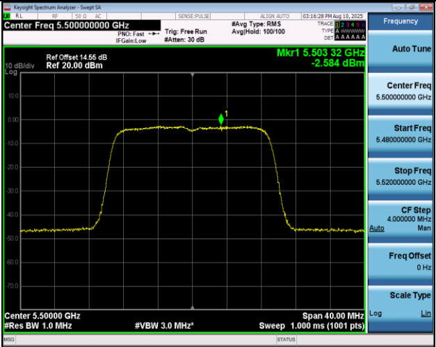
11AX20MIMO-Ant2-5500-PASS
