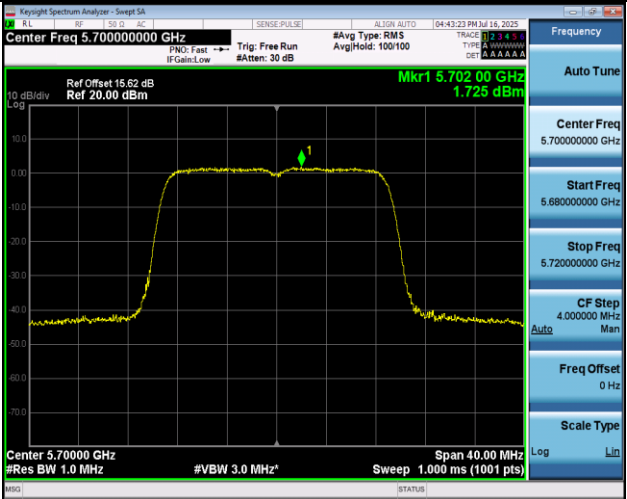
11N20MIMO-Ant2-5700-PASS
