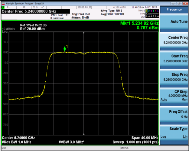
11AC20MIMO-Ant2-5240-PASS
