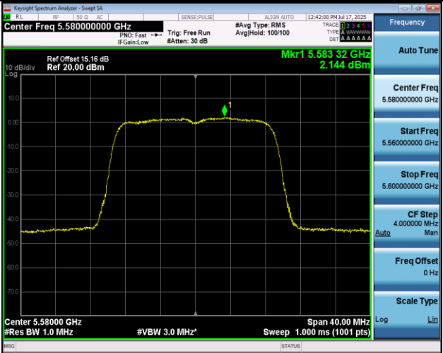
11AC20MIMO-Ant1-5580-PASS
