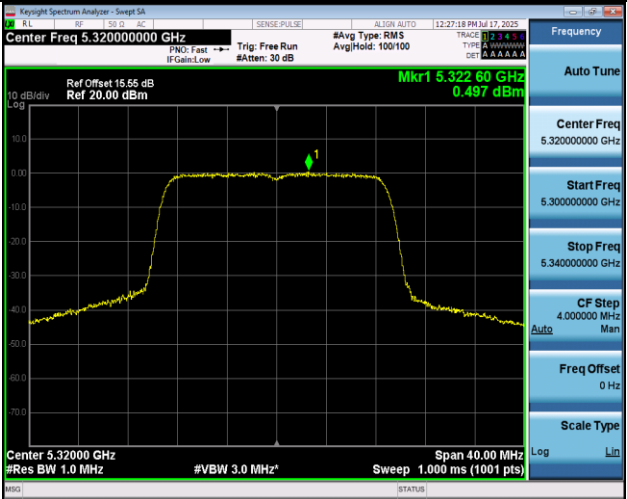
11AC20MIMO-Ant2-5320-PASS
