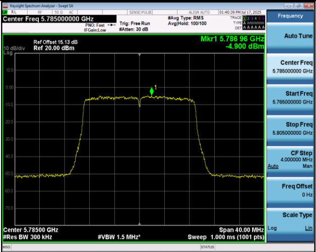
11AC20MIMO-Ant1-5785-PASS
