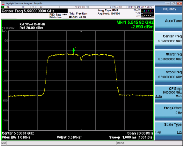
11N40MIMO-Ant2-5550-PASS
