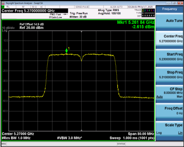
11AC40MIMO-Ant1-5270-PASS
