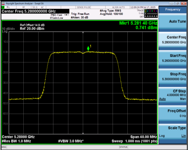
11AC20MIMO-Ant1-5280-PASS
