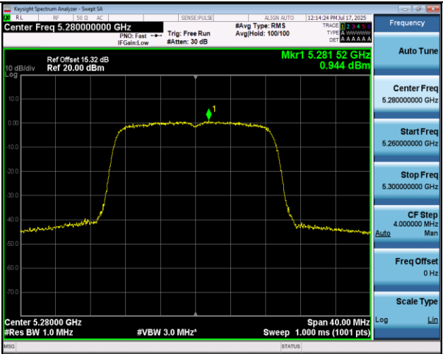
11AC20MIMO-Ant2-5280-PASS
