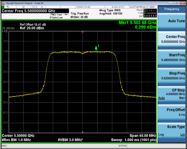
11AC20MIMO-Ant2-5500-PASS
