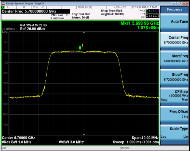
11AC20MIMO-Ant2-5700-PASS
