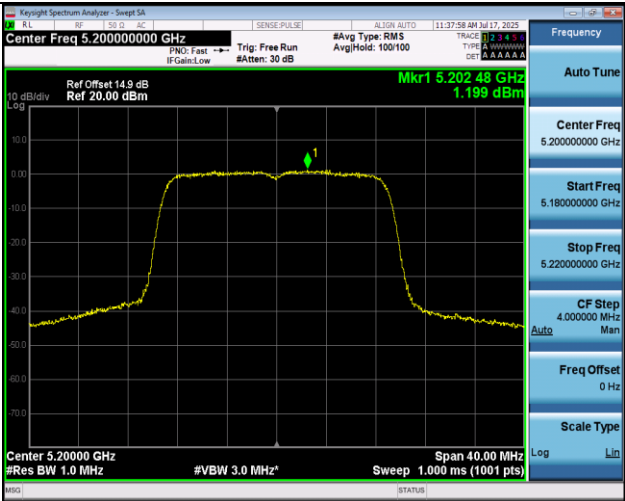
11AC20MIMO-Ant2-5200-PASS
