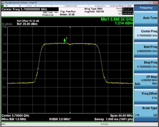
11AC20MIMO-Ant1-5700-PASS
