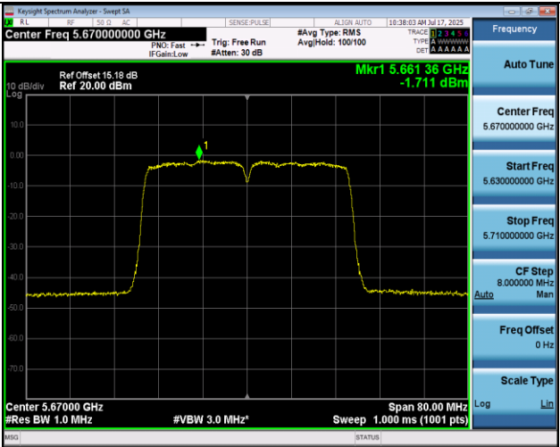
11N40MIMO-Ant1-5670-PASS
