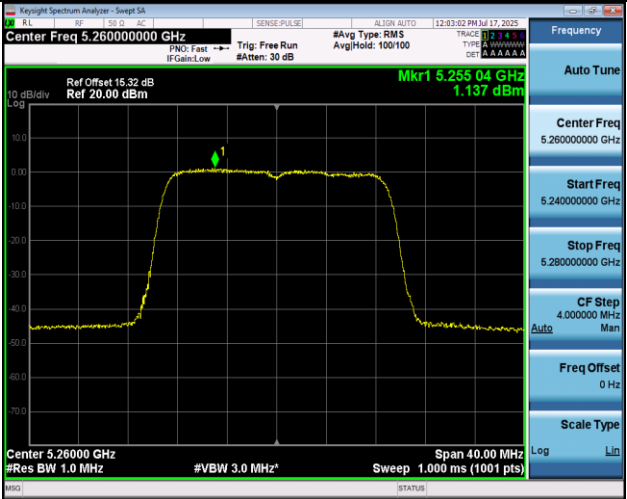
11AC20MIMO-Ant2-5260-PASS
