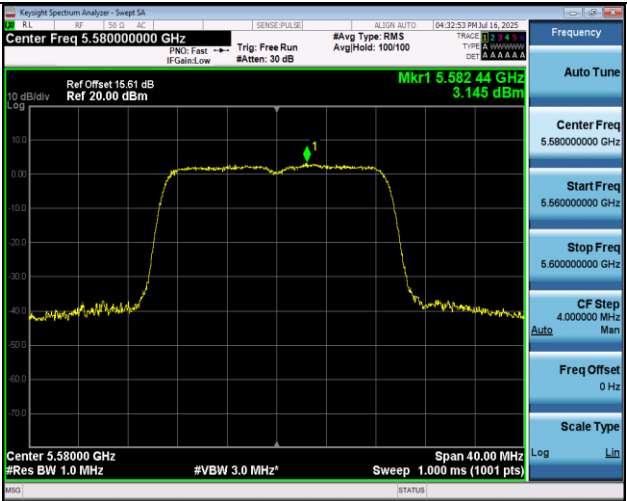
11N20MIMO-Ant2-5580-PASS
