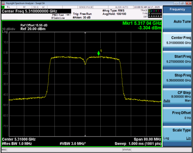
11N40MIMO-Ant2-5310-PASS
