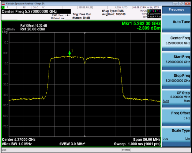
11N40MIMO-Ant2-5270-PASS
