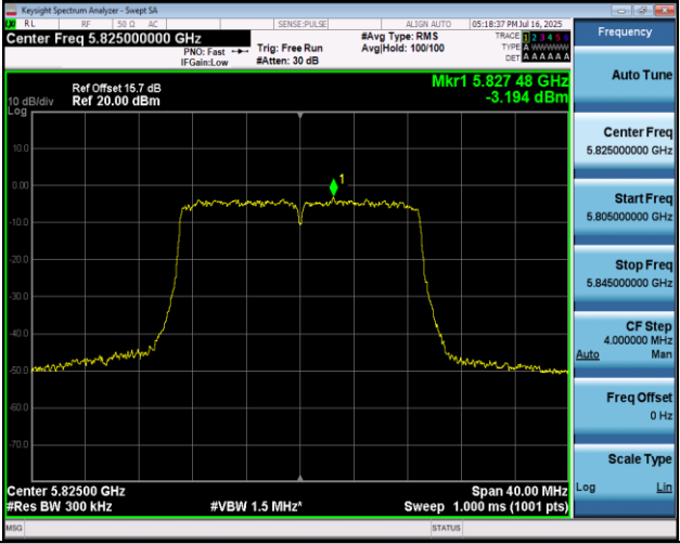
11N20MIMO-Ant2-5825-PASS
