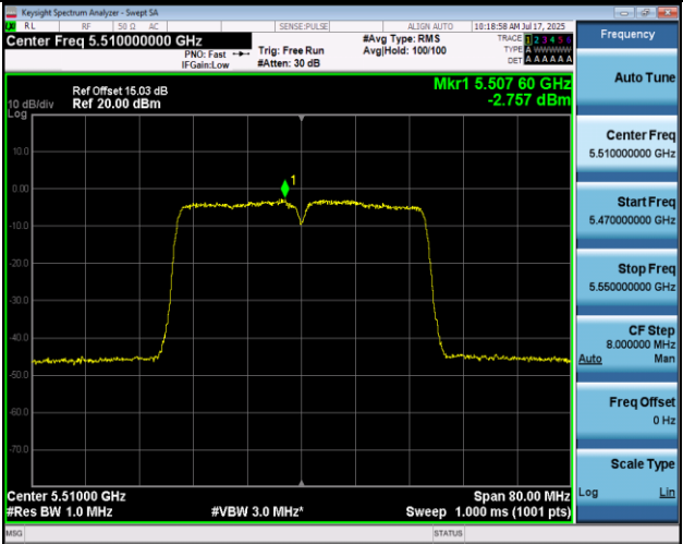
11N40MIMO-Ant1-5510-PASS
