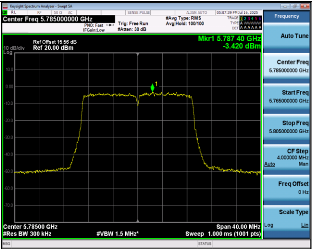
11N20MIMO-Ant2-5785-PASS
