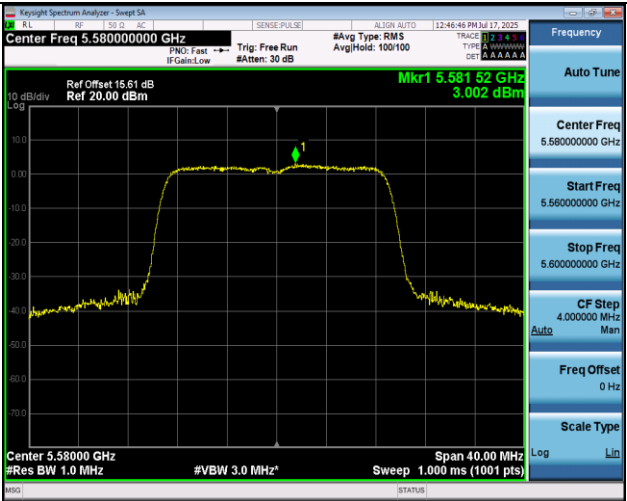
11AC20MIMO-Ant2-5580-PASS
