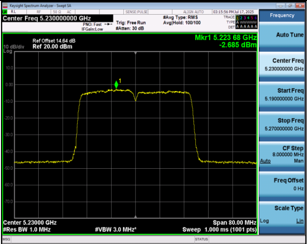
11AC40MIMO-Ant1-5230-PASS
