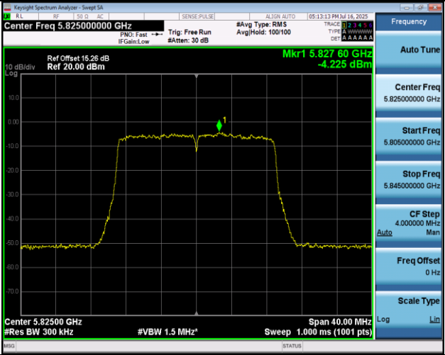
11N20MIMO-Ant1-5825-PASS
