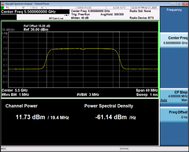
11AC20MIMO-Ant1-5500-PASS
