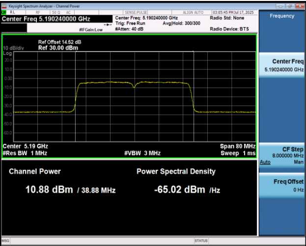
11AC40MIMO-Ant1-5190-PASS
