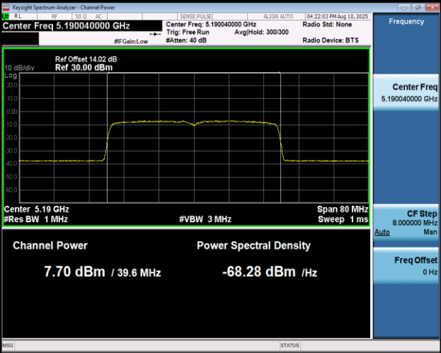
11AX40MIMO-Ant1-5190-PASS
