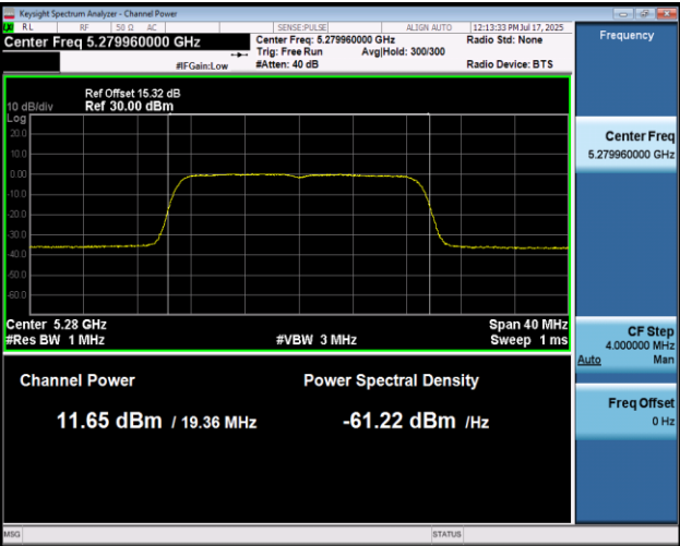
11AC20MIMO-Ant2-5280-PASS
