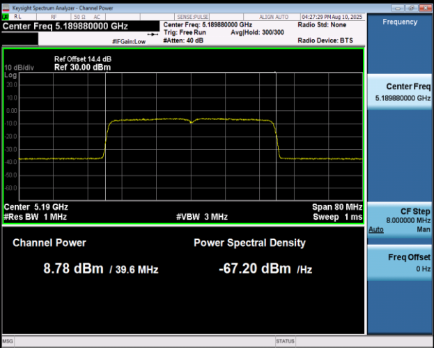
11AX40MIMO-Ant2-5190-PASS
