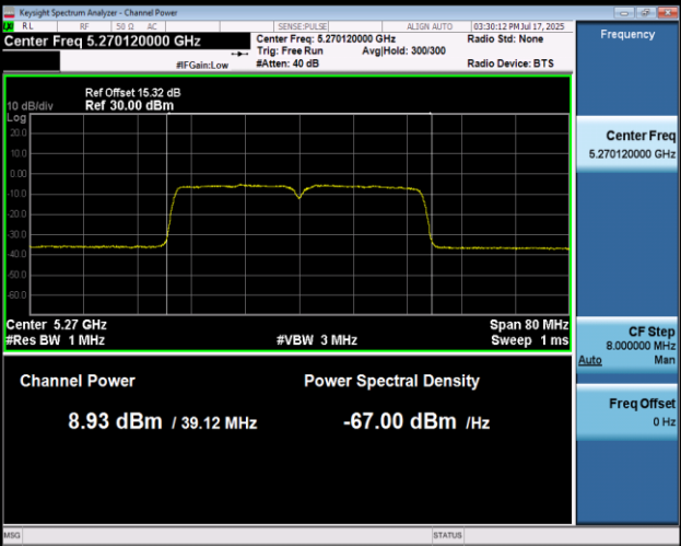
11AC40MIMO-Ant2-5270-PASS
