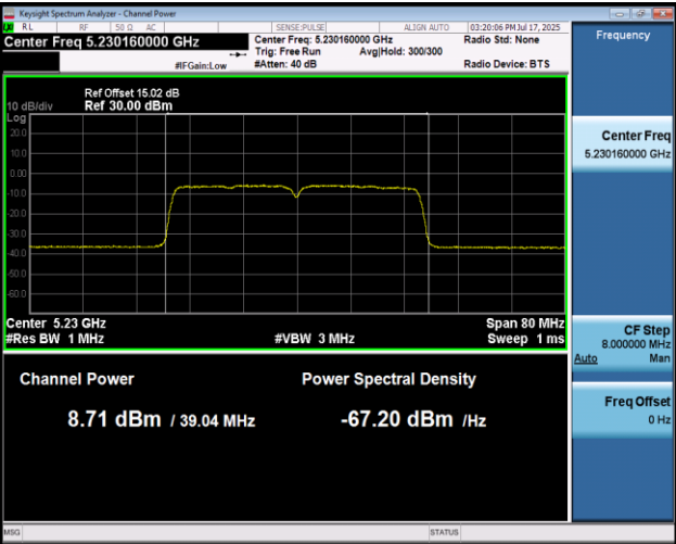
11AC40MIMO-Ant2-5230-PASS
