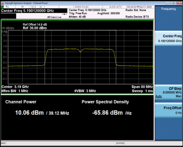
11AC40MIMO-Ant2-5190-PASS
