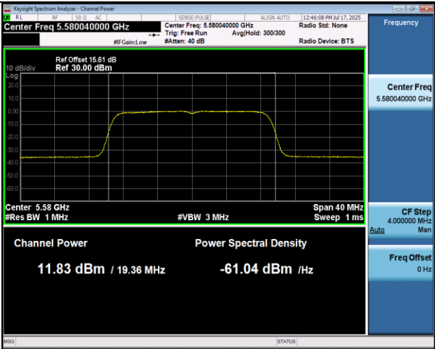
11AC20MIMO-Ant2-5580-PASS
