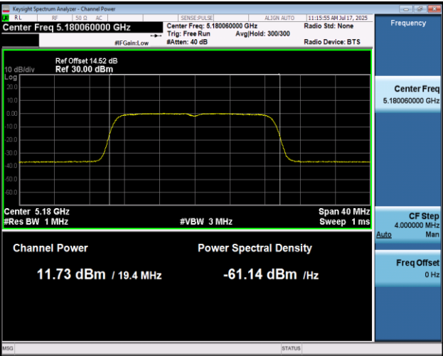
11AC20MIMO-Ant1-5180-PASS
