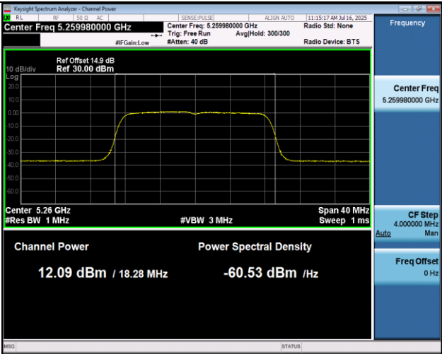
11A-Ant1-5260-PASS
