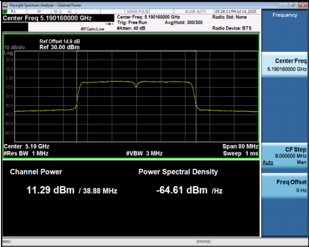
11N40MIMO-Ant2-5190-PASS
