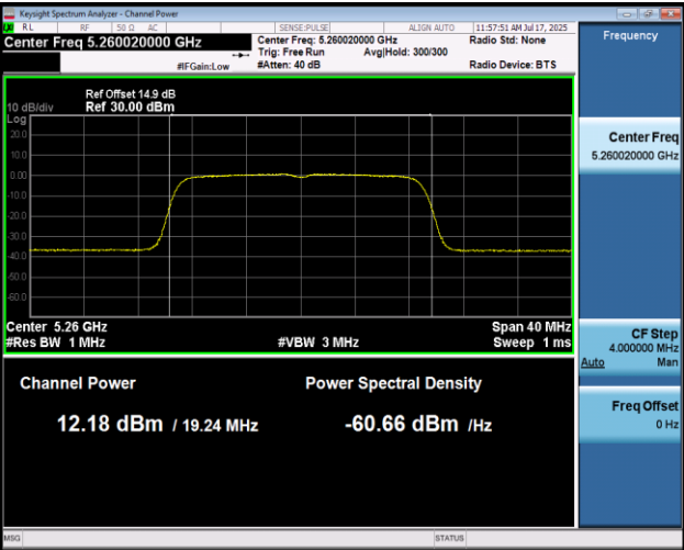
11AC20MIMO-Ant1-5260-PASS
