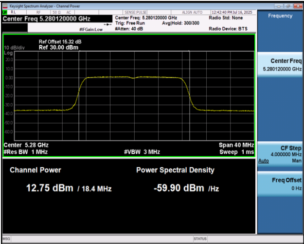
11A-Ant2-5280-PASS
