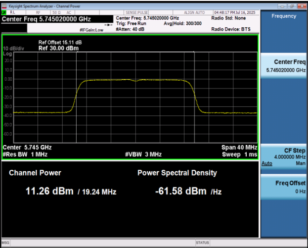
11N20MIMO-Ant1-5745-PASS
