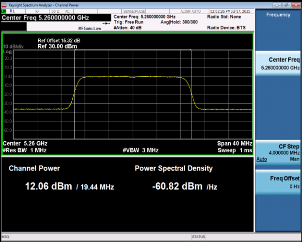
11AC20MIMO-Ant2-5260-PASS
