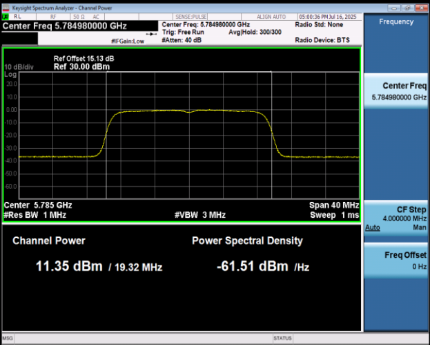
11N20MIMO-Ant1-5785-PASS
