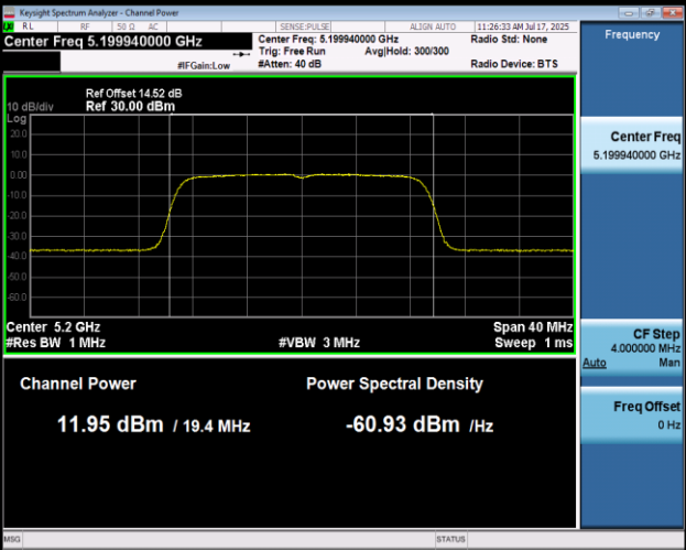
11AC20MIMO-Ant1-5200-PASS
