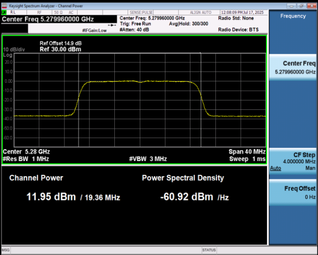
11AC20MIMO-Ant1-5280-PASS
