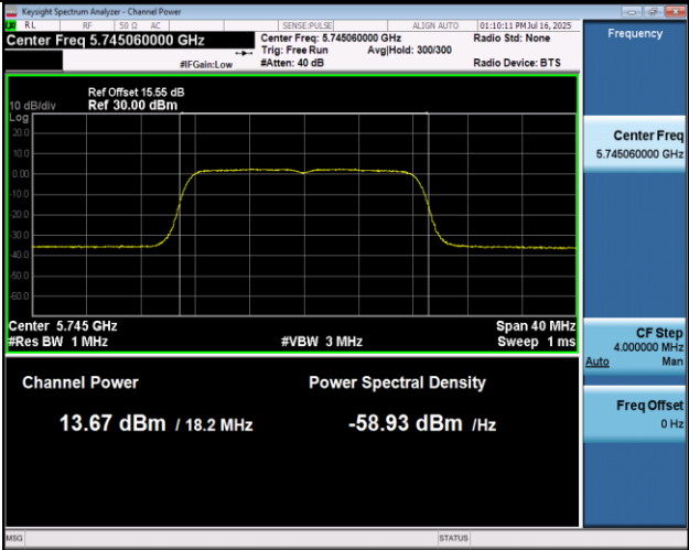
11A-Ant2-5745-PASS
