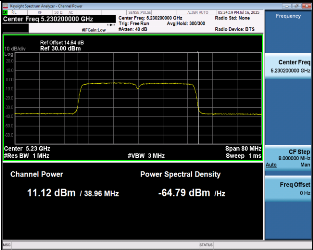
11N40MIMO-Ant1-5230-PASS
