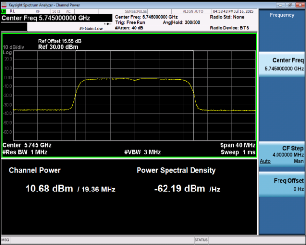
11N20MIMO-Ant2-5745-PASS
