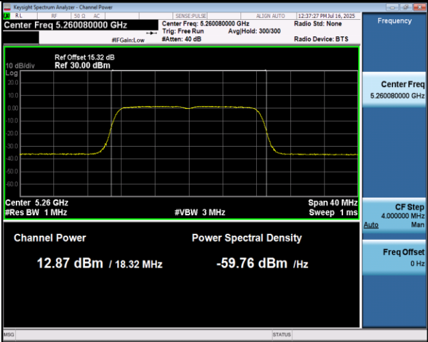
11A-Ant2-5260-PASS
