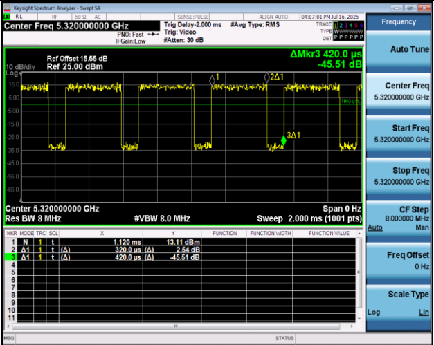
NTNV-11N20MIMO-Ant2-5320
