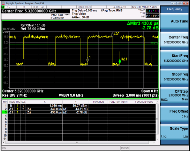
NTNV-11AC20MIMO-Ant1-5320
