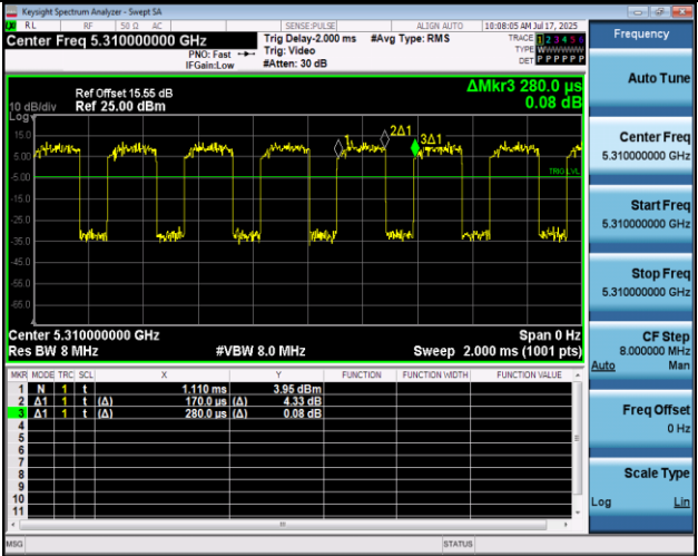
NTVN-11N40MIMO-Ant2-5310
