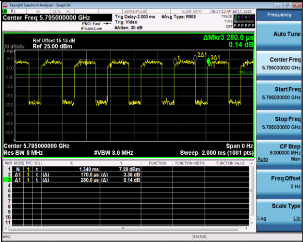
NTVN-11N40MIMO-Ant1-5795
