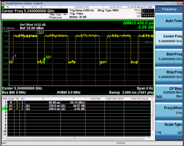
NTNV-11AC20MIMO-Ant2-5240
