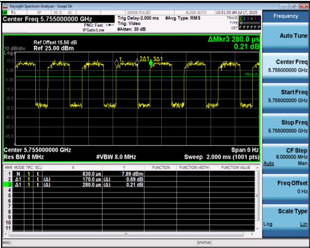
NTVN-11N40MIMO-Ant2-5755
