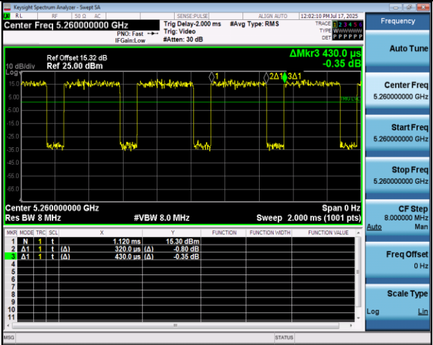
NTNV-11AC20MIMO-Ant2-5260
