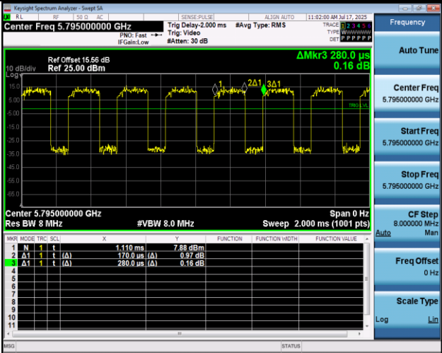
NTVN-11N40MIMO-Ant2-5795
