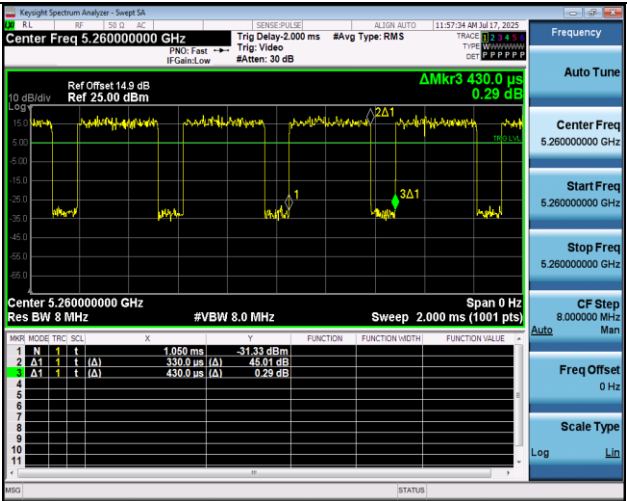
NTNV-11AC20MIMO-Ant1-5260
