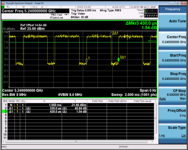
NTNV-11AC20MIMO-Ant1-5240
