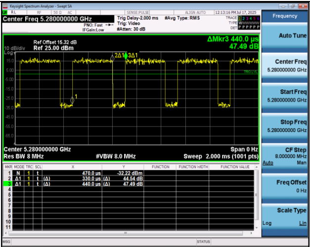
NTNV-11AC20MIMO-Ant2-5280
