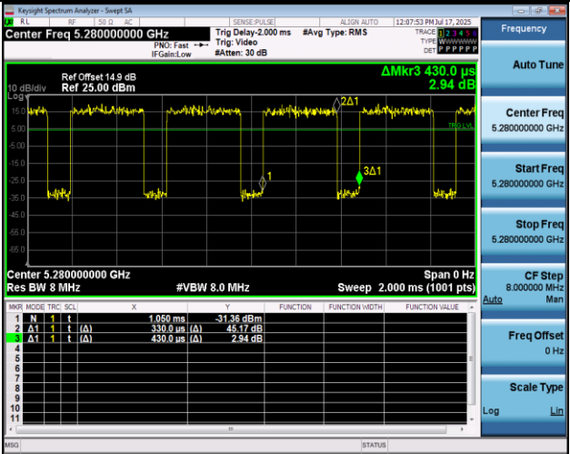
NTNV-11AC20MIMO-Ant1-5280
