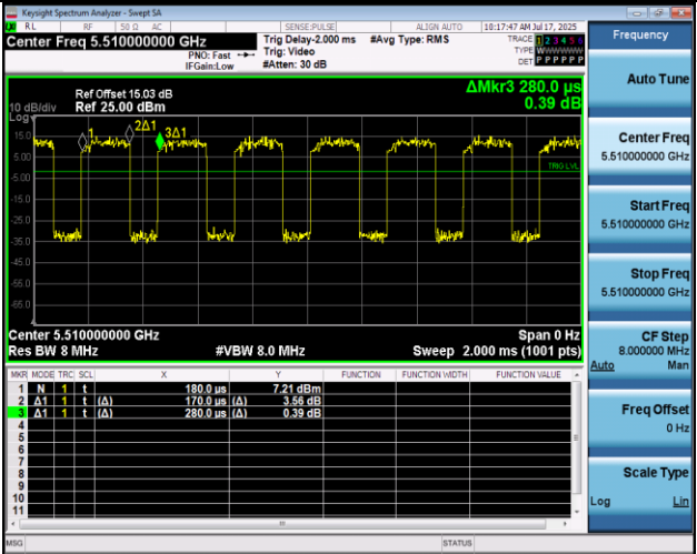
NTVN-11N40MIMO-Ant1-5510
