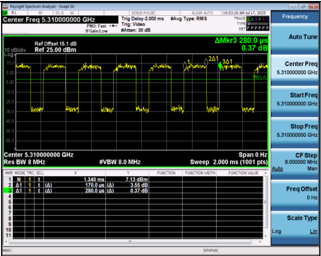
NTVN-11N40MIMO-Ant1-5310
