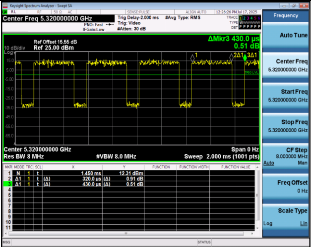
NTNV-11AC20MIMO-Ant2-5320
