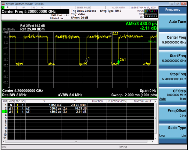
NTNV-11AC20MIMO-Ant2-5200
