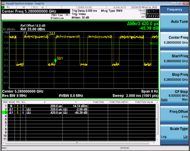
NTVN-11N20MIMO-Ant1-5280
