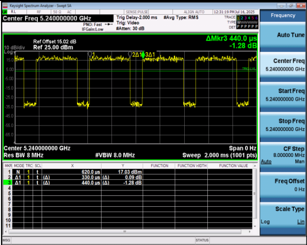
NTNV-11A-Ant2-5240
