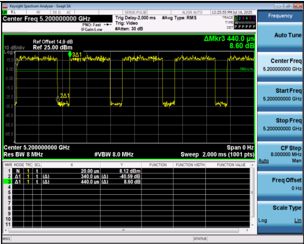
NTNV-11A-Ant2-5200
