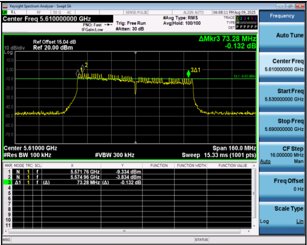
11AC80MIMO-Ant2-5610-PASS
