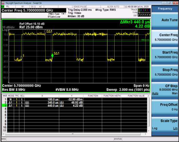
NTNV-11A-Ant1-5700
