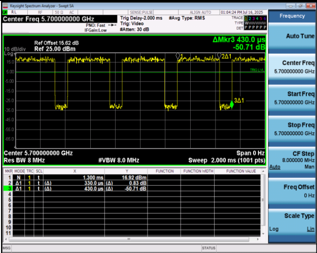
NTNV-11A-Ant2-5700
