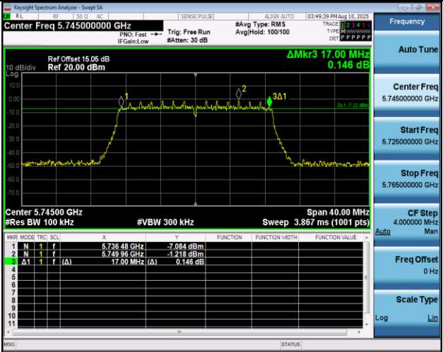
11AX20MIMO-Ant2-5745-PASS
