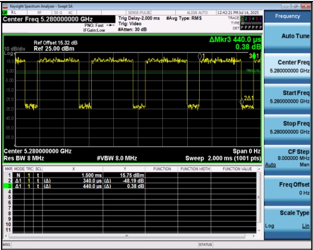
NTNV-11A-Ant2-5280
