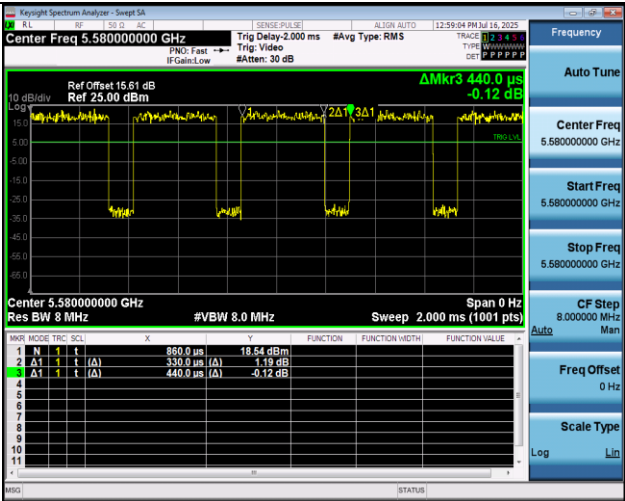
NTNV-11A-Ant2-5580
