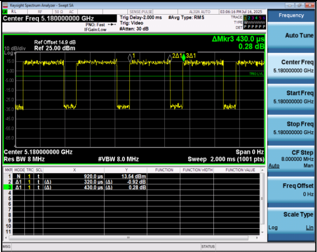
NTNV-11N20MIMO-Ant2-5180
