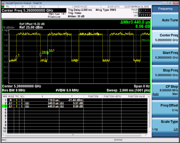
NTNV-11A-Ant2-5260
