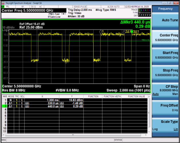
NTNV-11A-Ant2-5500
