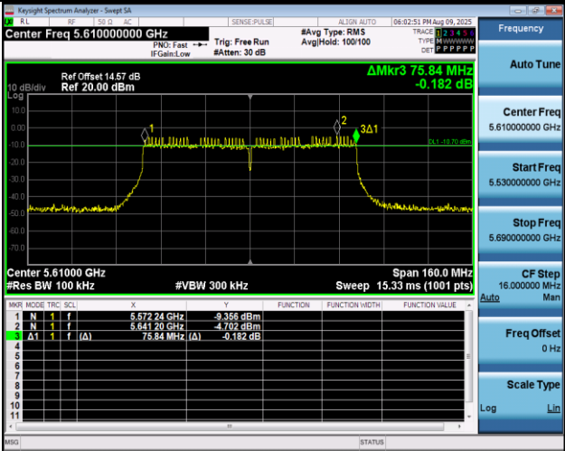
11AC80MIMO-Ant1-5610-PASS
