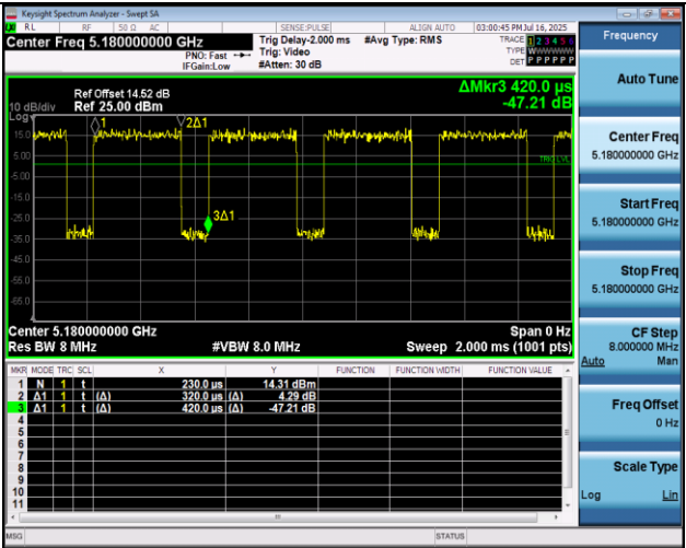
NTNV-11N20MIMO-Ant1-5180
