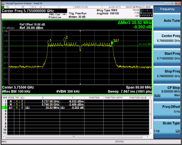
11AC40MIMO-Ant2-5755-PASS
