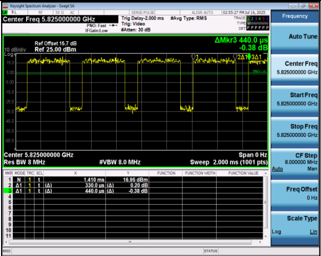
NTNV-11A-Ant2-5825
