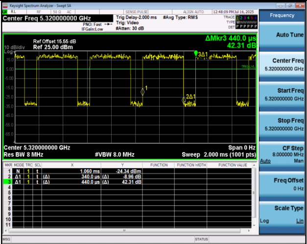
NTNV-11A-Ant2-5320
