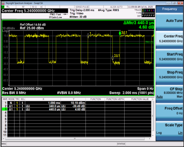
NTNV-11A-Ant1-5240
