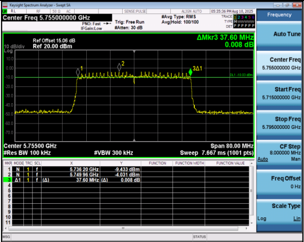
11AX40MIMO-Ant2-5755-PASS
