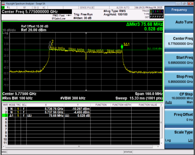
11AC80MIMO-Ant2-5775-PASS
