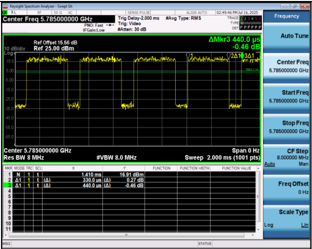
NTNV-11A-Ant2-5785
