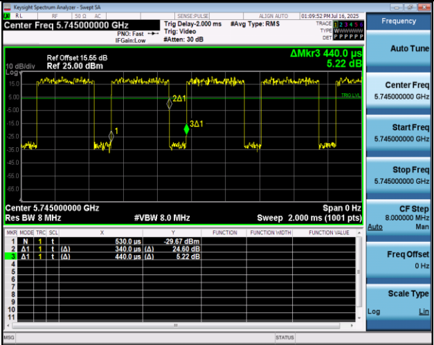
NTNV-11A-Ant2-5745
