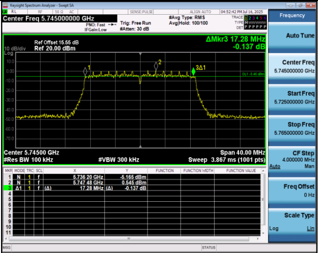
11N20MIMO-Ant2-5745-PASS
