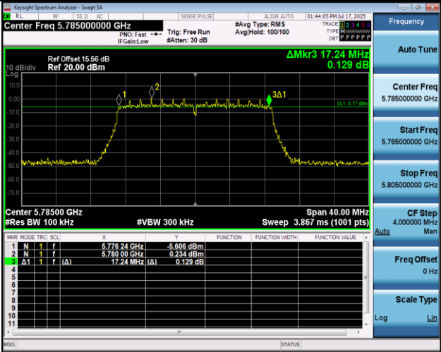
11AC20MIMO-Ant2-5785-PASS
