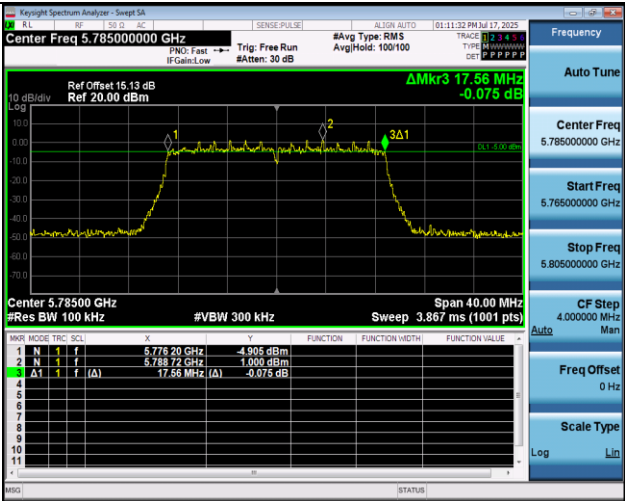
11AC20MIMO-Ant1-5785-PASS
