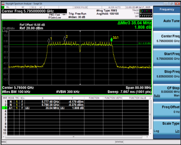
11N40MIMO-Ant2-5795-PASS
