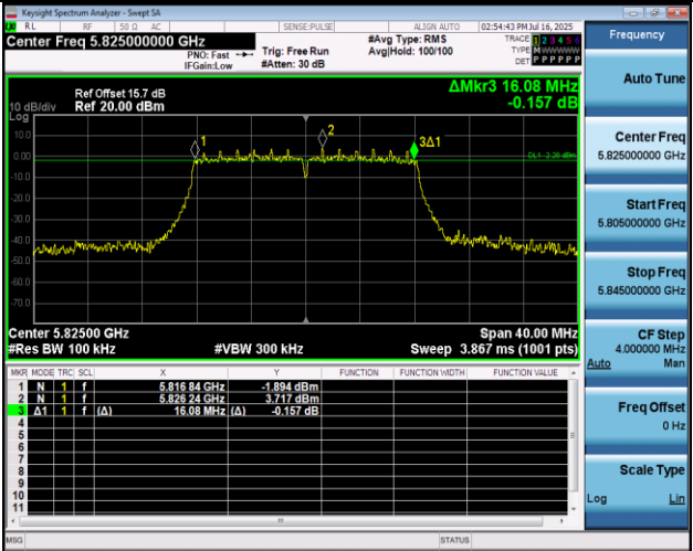
11A-Ant2-5825-PASS
