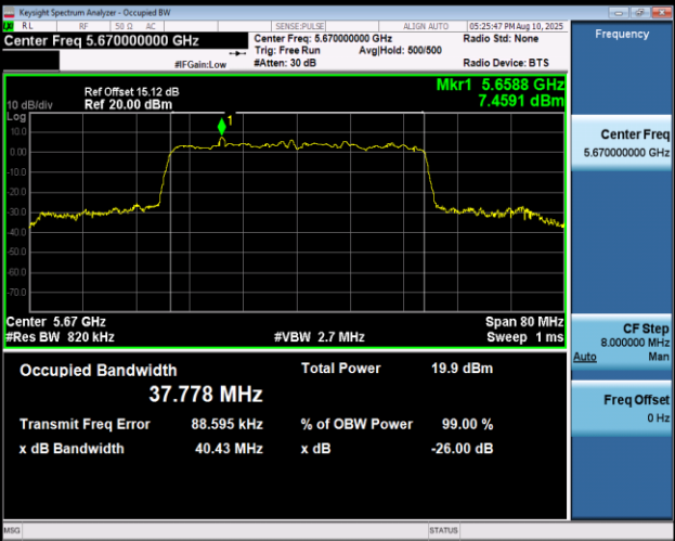
11AX40MIMO-Ant2-5670
