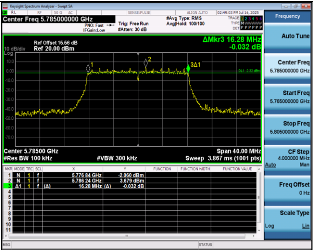
11A-Ant2-5785-PASS
