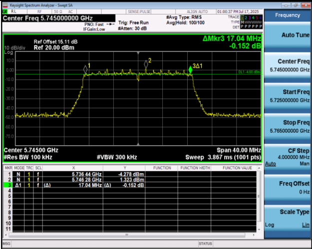
11AC20MIMO-Ant1-5745-PASS
