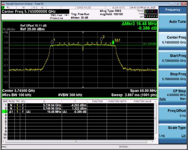
11N20MIMO-Ant1-5745-PASS
