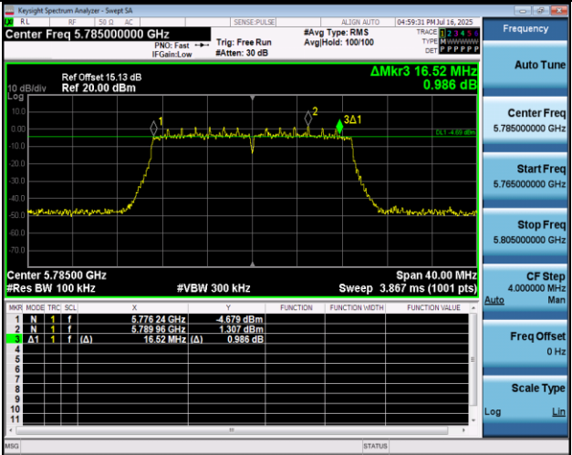
11N20MIMO-Ant1-5785-PASS
