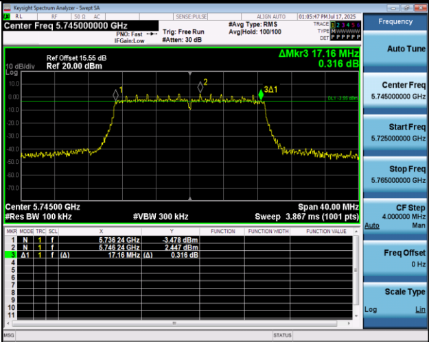
11AC20MIMO-Ant2-5745-PASS
