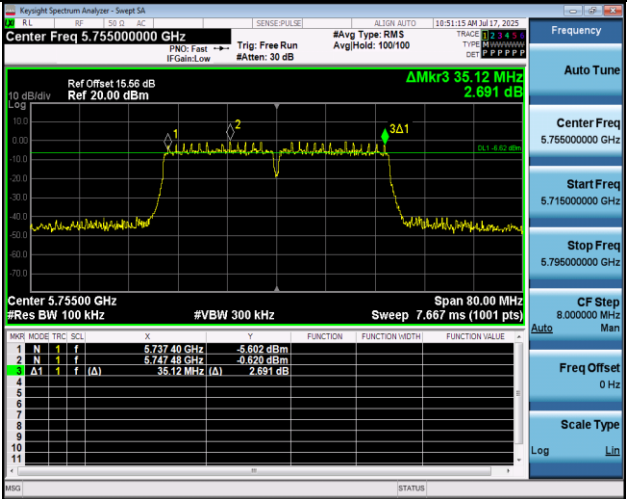
11N40MIMO-Ant2-5755-PASS
