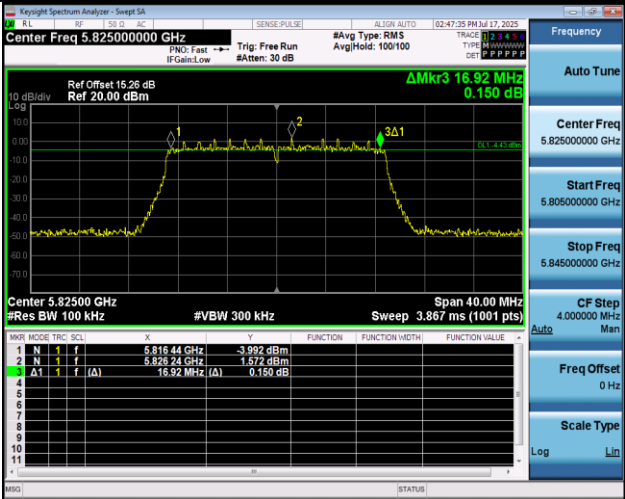
11AC20MIMO-Ant1-5825-PASS
