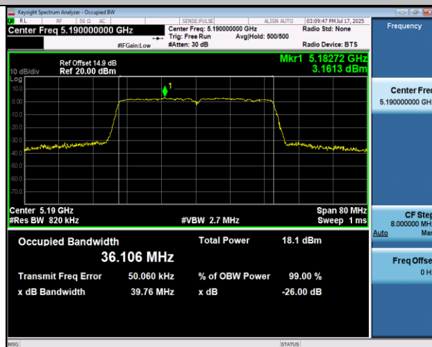
11AC40MIMO-Ant2-5190
