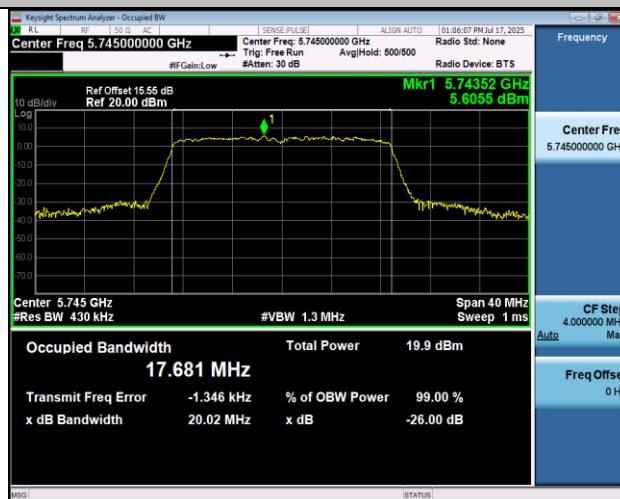
11AC20MIMO-Ant2-5745
