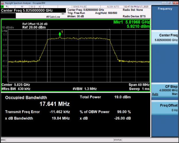
11AC20MIMO-Ant1-5825
