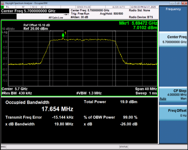
11AC20MIMO-Ant1-5700
