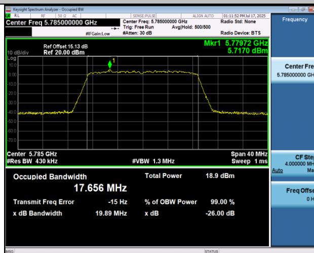
11AC20MIMO-Ant1-5785
