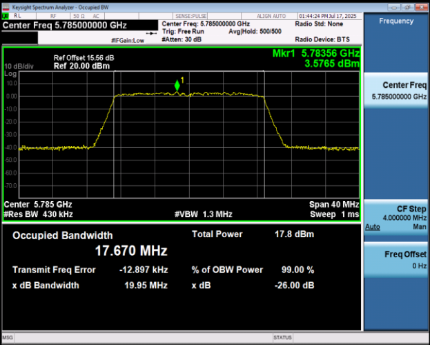
11AC20MIMO-Ant2-5785
