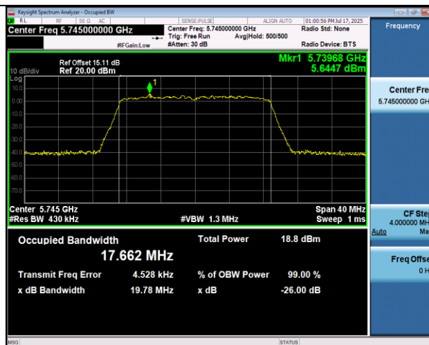
11AC20MIMO-Ant1-5745
