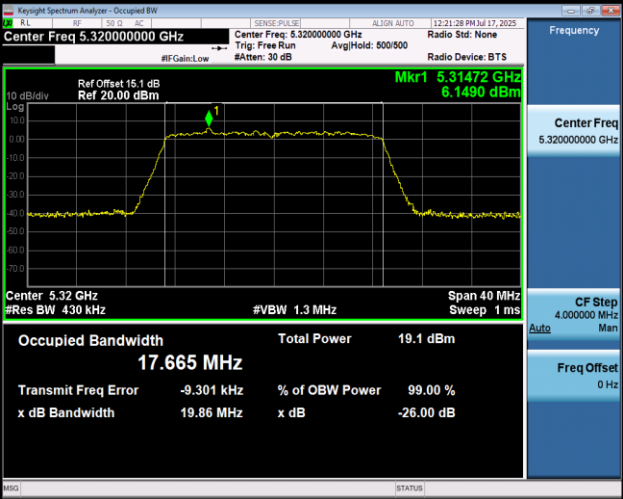
11AC20MIMO-Ant1-5320
