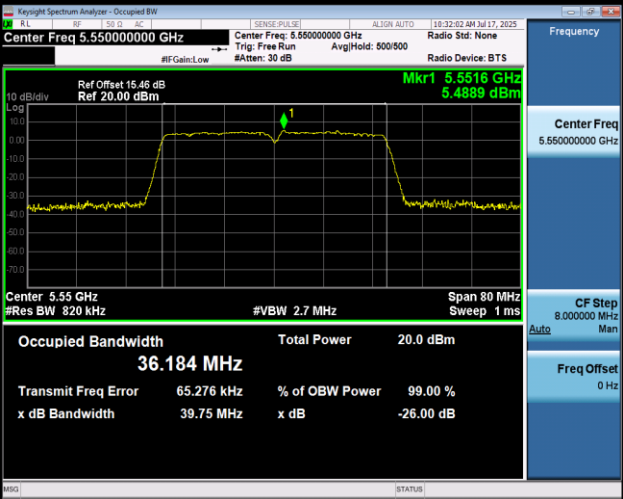
11N40MIMO-Ant2-5550
