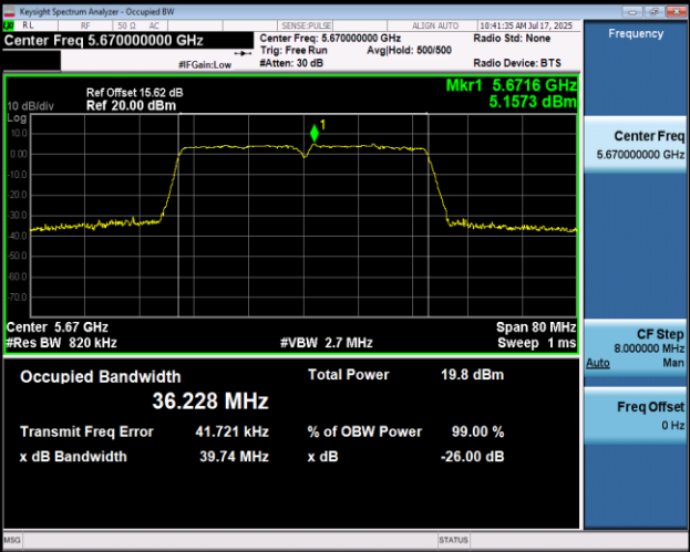
11N40MIMO-Ant2-5670
