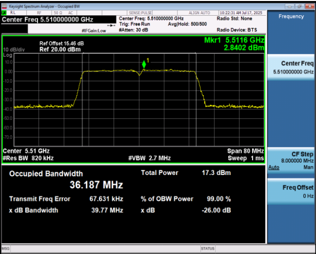
11N40MIMO-Ant2-5510
