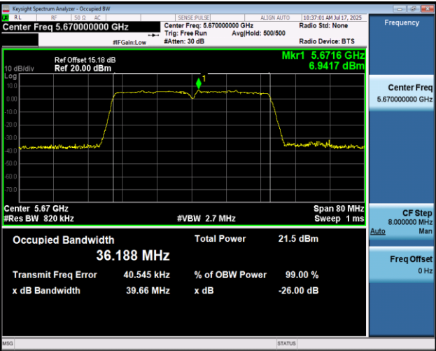
11N40MIMO-Ant1-5670
