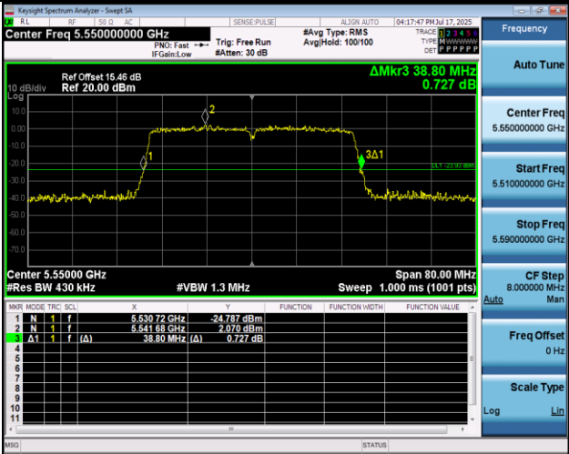
11AC40MIMO-Ant2-5550
