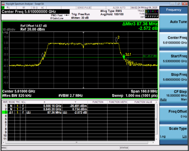
11AC80MIMO-Ant1-5610
