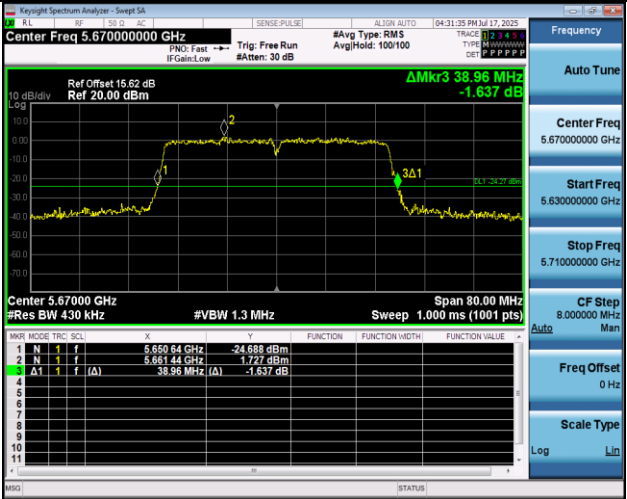
11AC40MIMO-Ant2-5670
