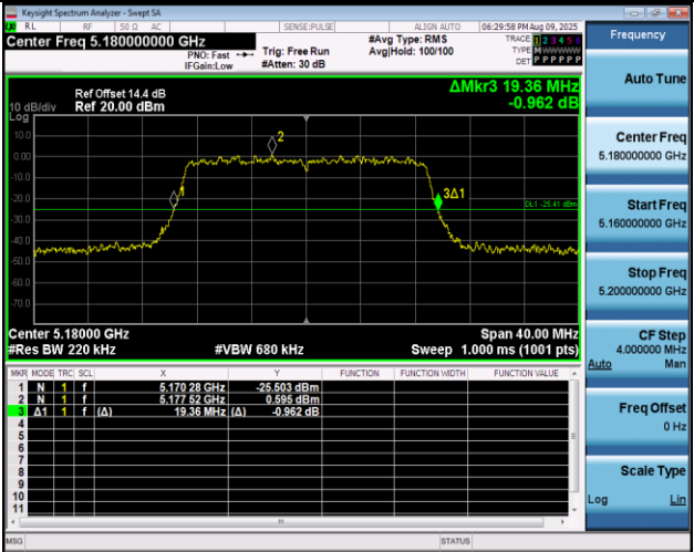
11AX20MIMO-Ant2-5180
