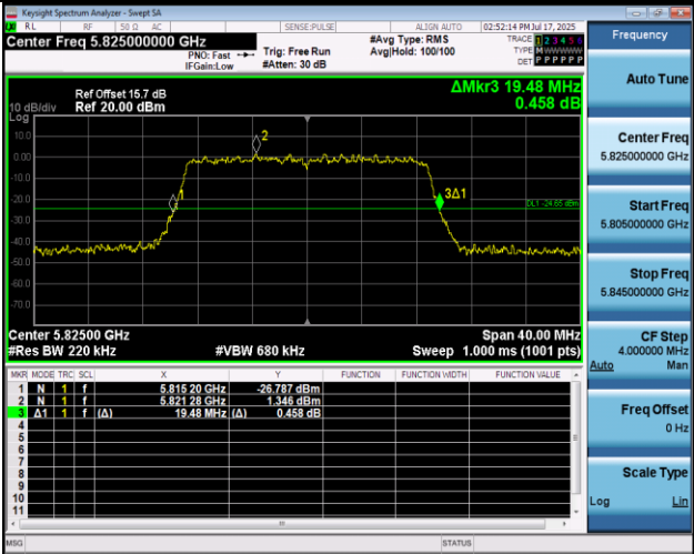
11AC20MIMO-Ant2-5825
