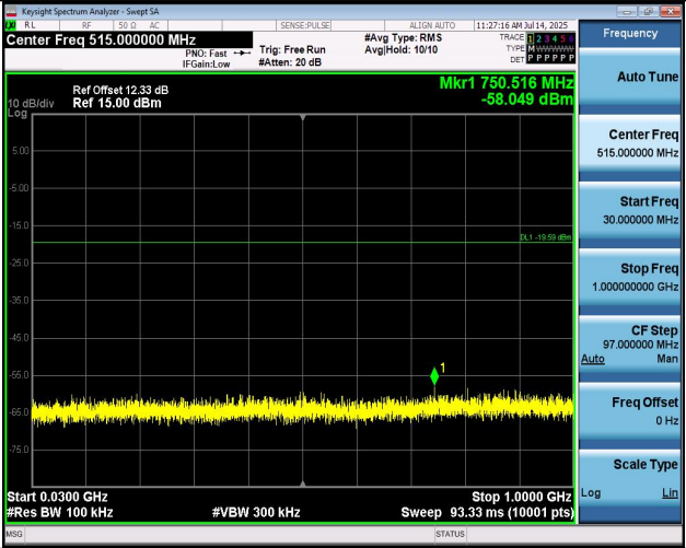
11AX40MIMO-Ant2-2452-30~1000-PASS
