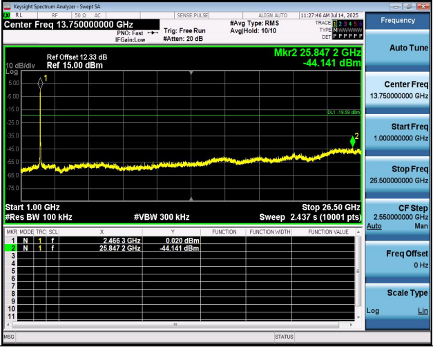
11AX40MIMO-Ant2-2452-1000~26500-PASS
