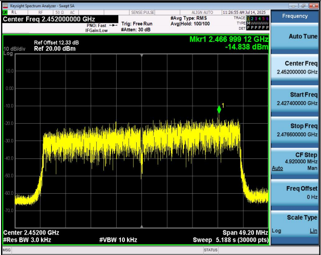
11AX40MIMO-Ant2-2452-PASS
