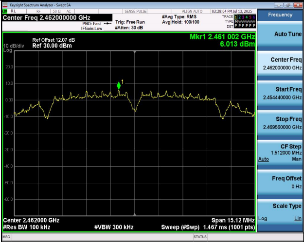
11B-Ant1-2462-PASS
