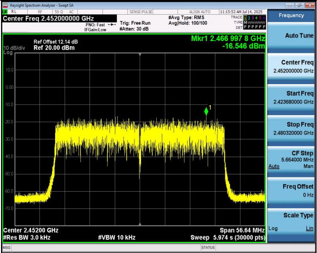
11AX40MIMO-Ant1-2452-PASS
