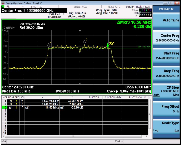
11N20MIMO-Ant1-2462-PASS
