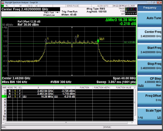
11G-Ant2-2462-PASS
