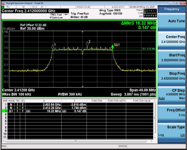
11G-Ant2-2412-PASS
