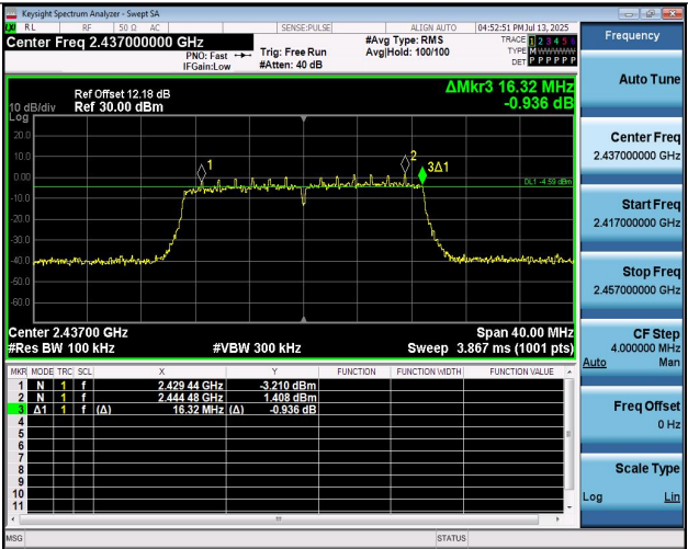
11N20MIMO-Ant2-2437-PASS
