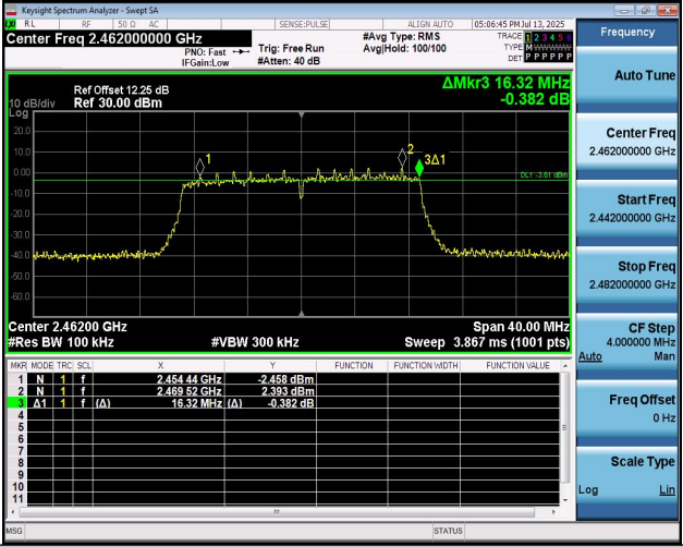
11N20MIMO-Ant2-2462-PASS
