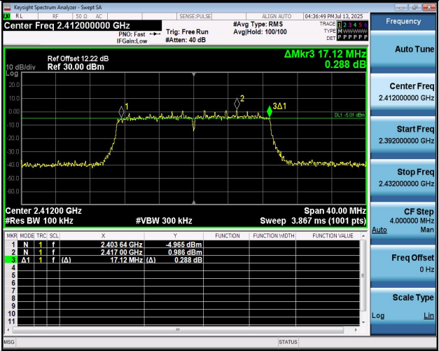
11N20MIMO-Ant2-2412-PASS
