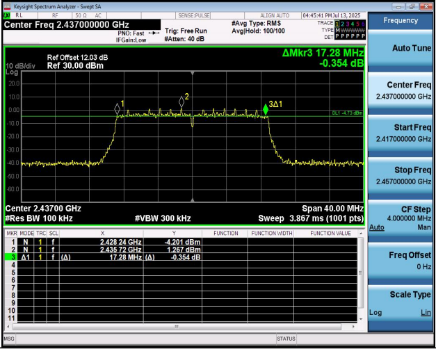
11N20MIMO-Ant1-2437-PASS
