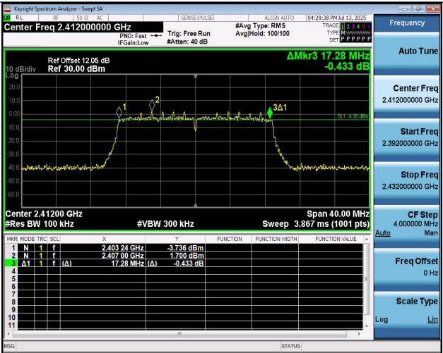
11N20MIMO-Ant1-2412-PASS
