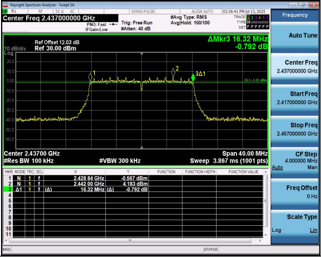
11G-Ant1-2437-PASS
