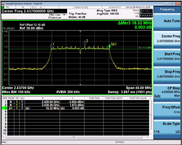
11G-Ant2-2437-PASS
