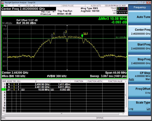
11B-Ant1-2462-PASS
