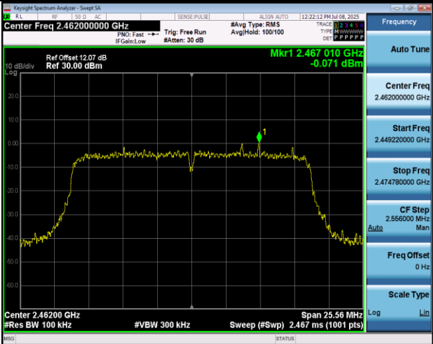
11N20SISO-Ant1-2462-PASS
