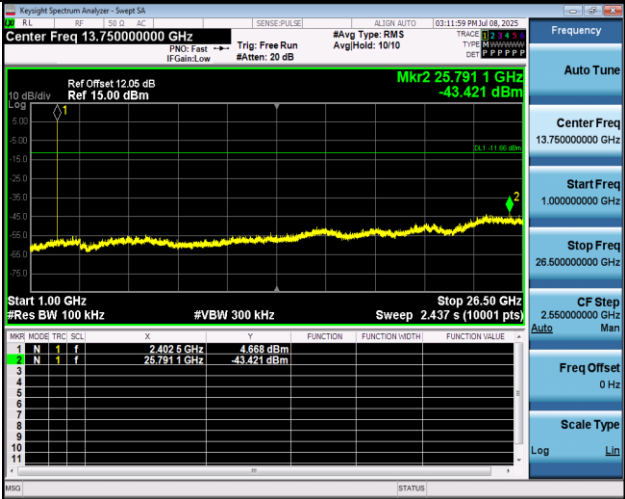
LE_2M-Ant1-2402-1000~26500-PASS
