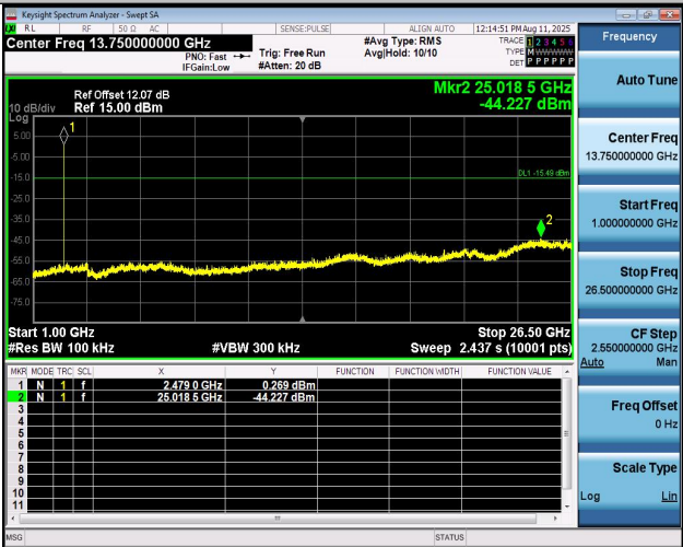
2DH5-Ant1-2480-1000~26500-PASS
