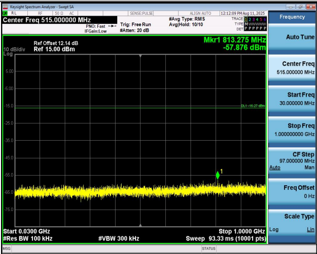
2DH5-Ant1-2441-30~1000-PASS
