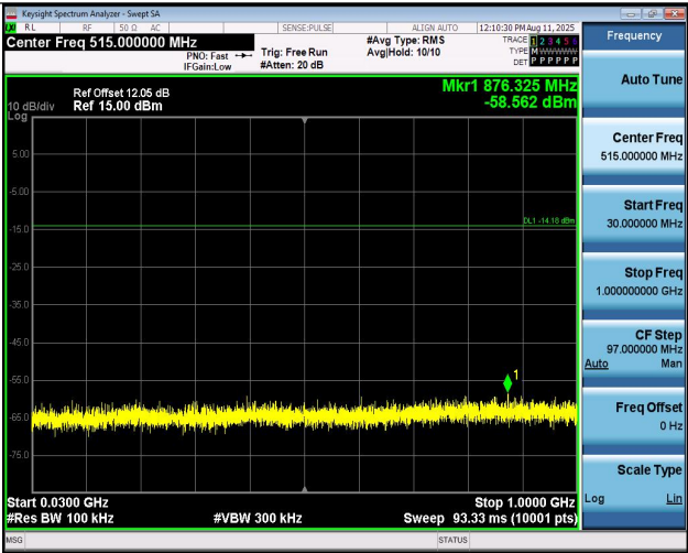
2DH5-Ant1-2402-30~1000-PASS
