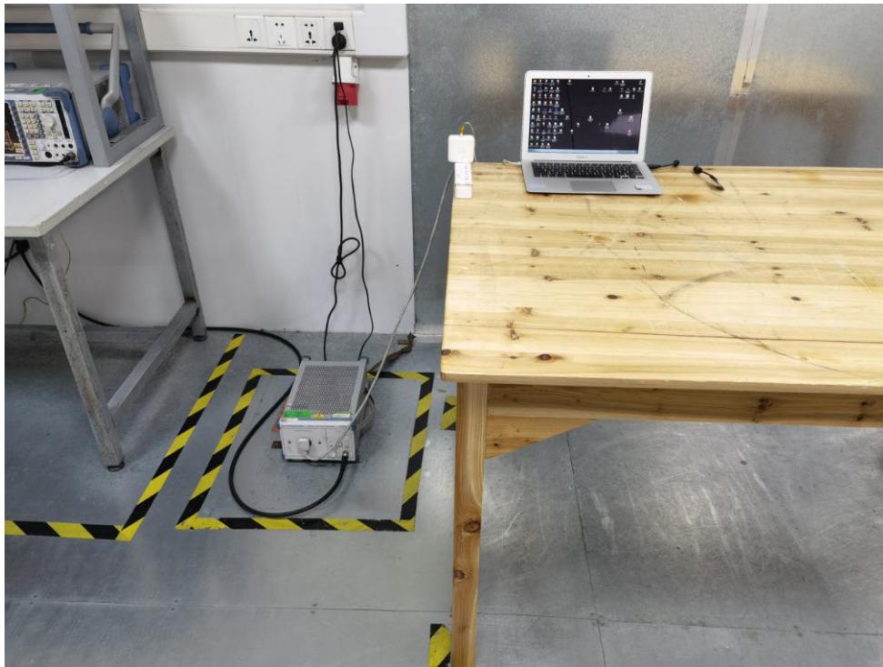
FCC ID: 2A2P9-ESP-M2 Photo of Power Line Conducted Emission Test
