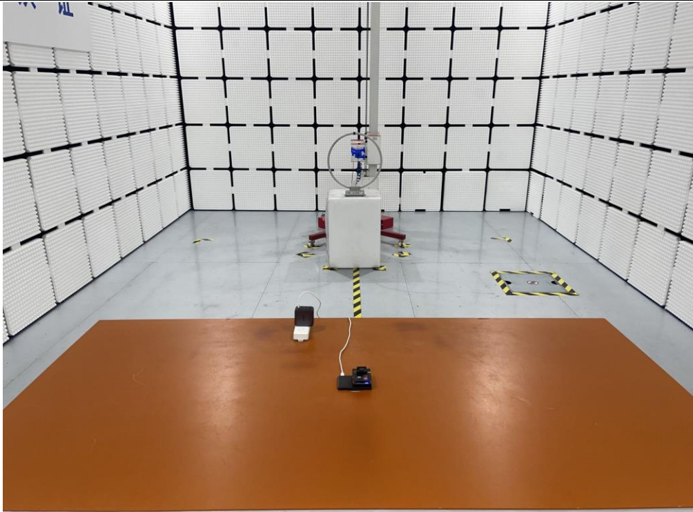
Radiated Emission Below 30MHz
